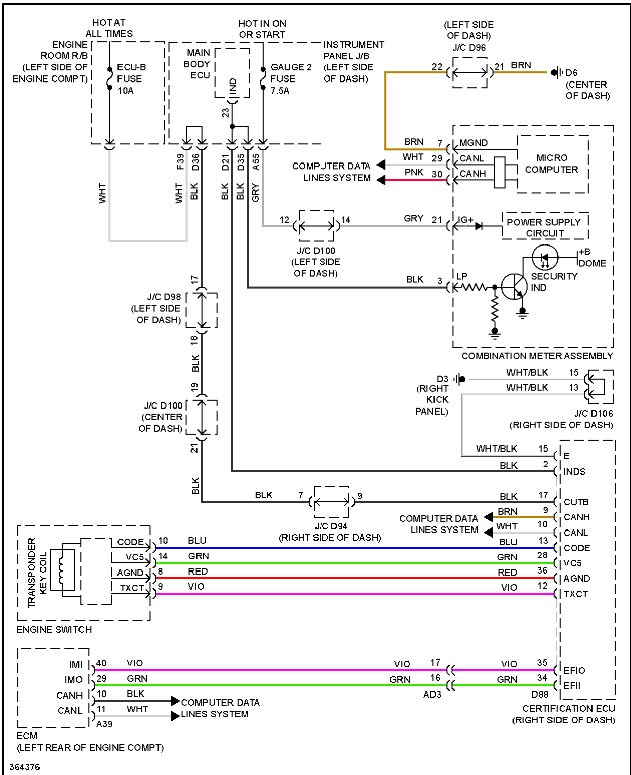
Fig. 11: Immobilizer Circuit, W/ Smart Key System
