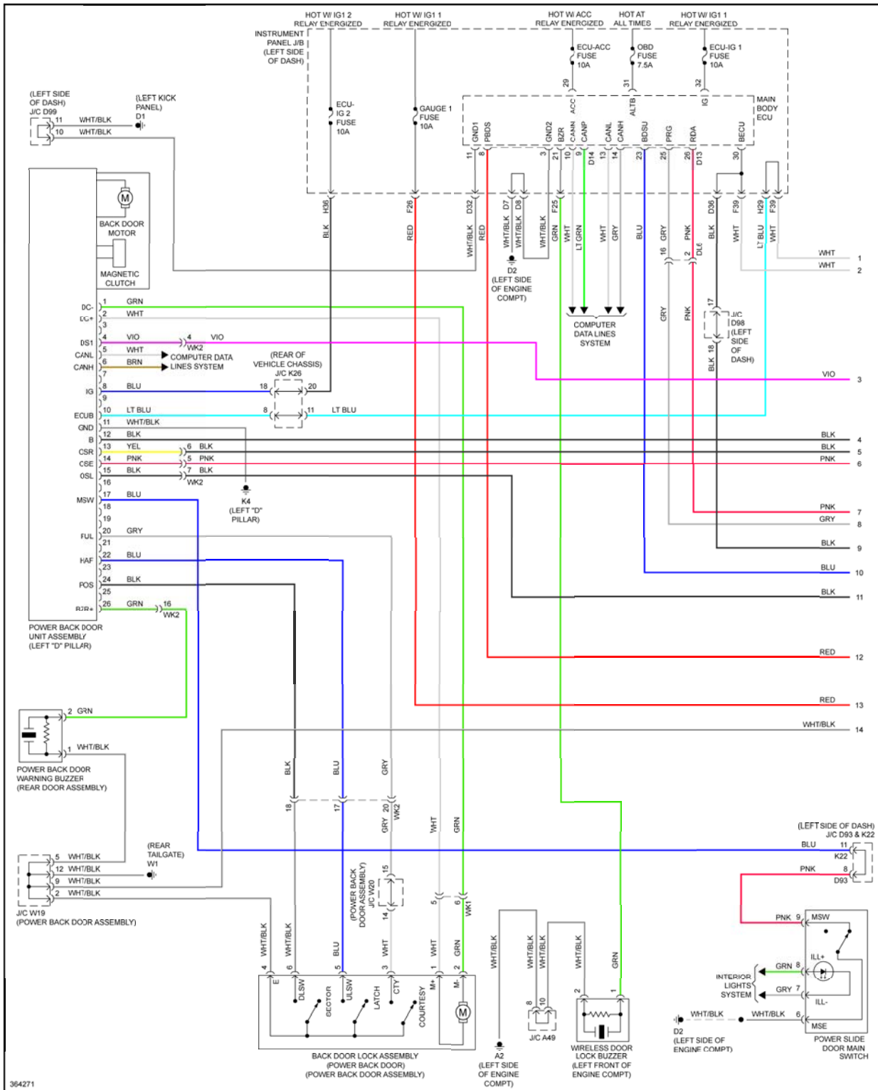
Fig. 117: Back Door Opener Circuit, W/ Power Back Door (1 of 2)
