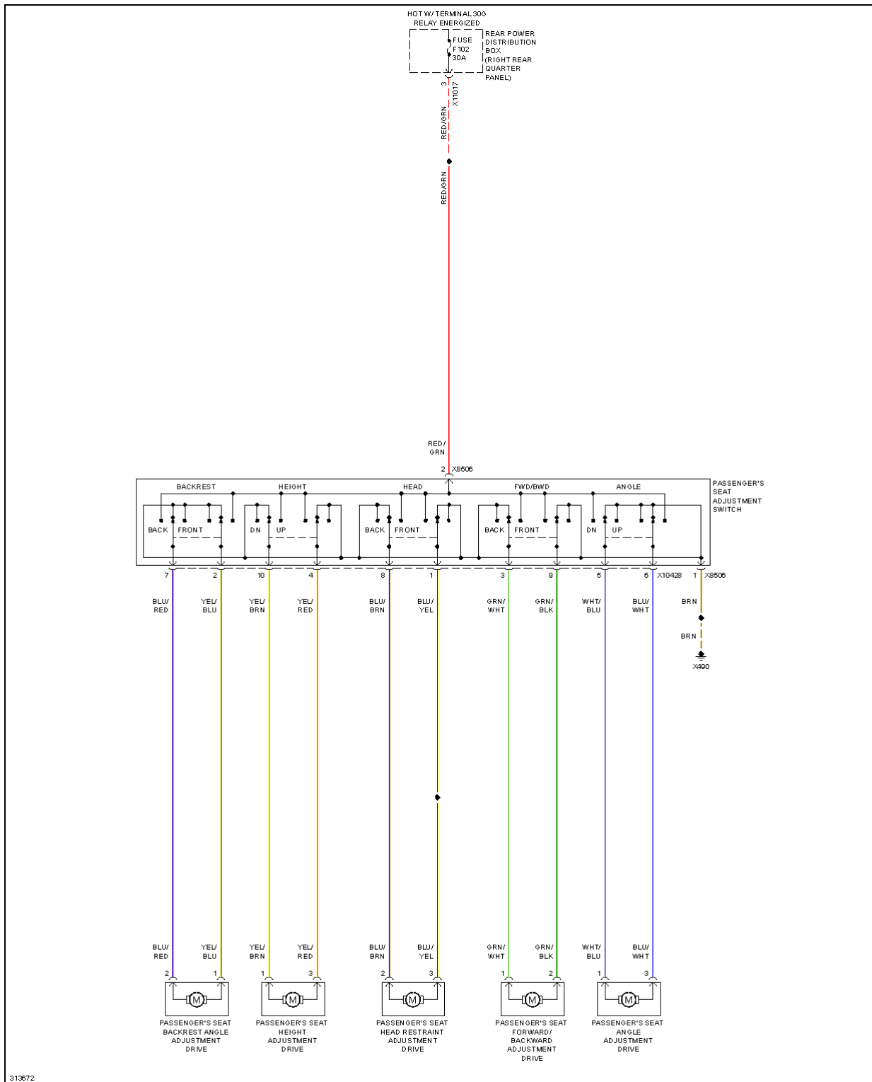
Fig. 96: Power Seats Circuit, W/ Passenger Power Seats
