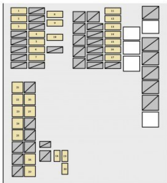
Scion xB mk2 – fuse box – engine compartment
