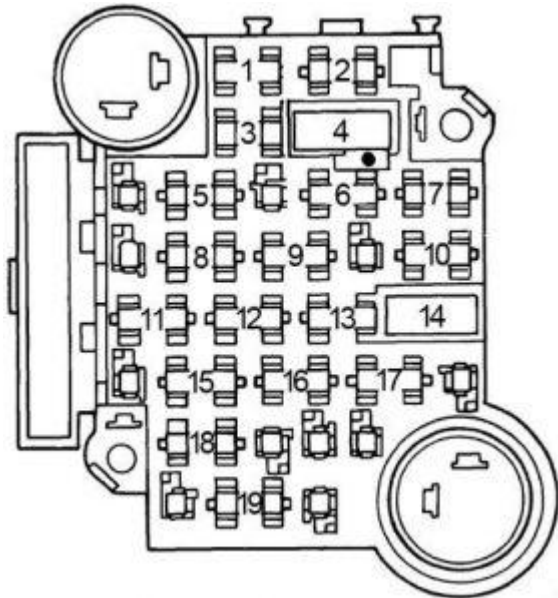
Pontiac Grand Am – fuse box diagram
