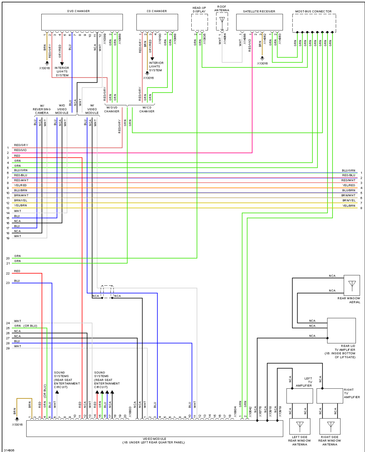
Fig. 68: Navigation Circuit, W/ CCC & M-ASK (2 of 3)
