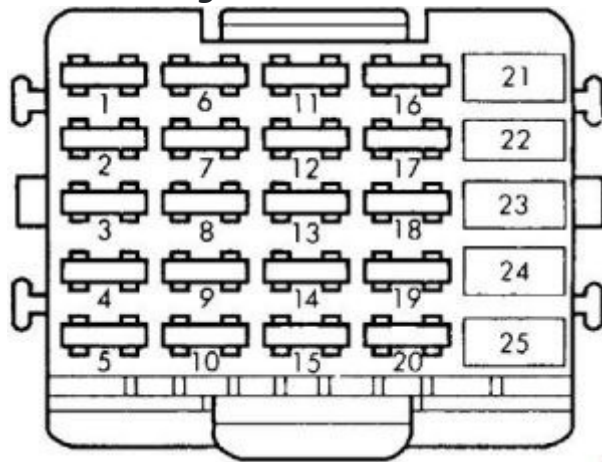
Chevrolet Caprice – fuse box diagram
