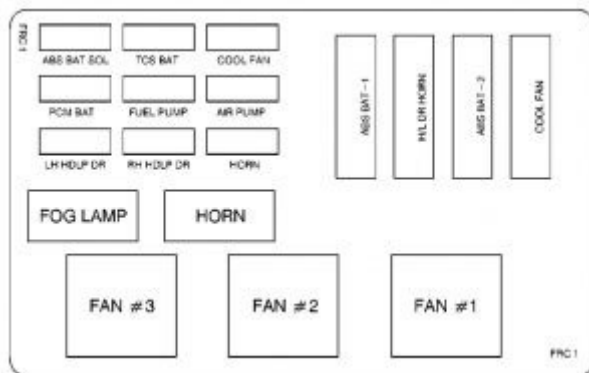
Pontiac Firebird – fuse box – engine compartment
