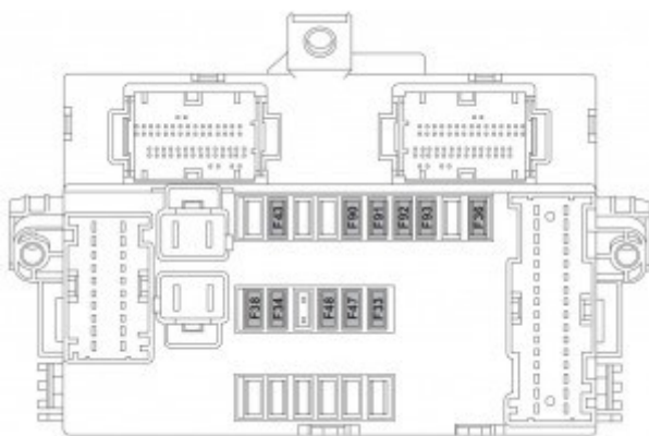
Fiat 500L LIVING – fuse box – dashboard
