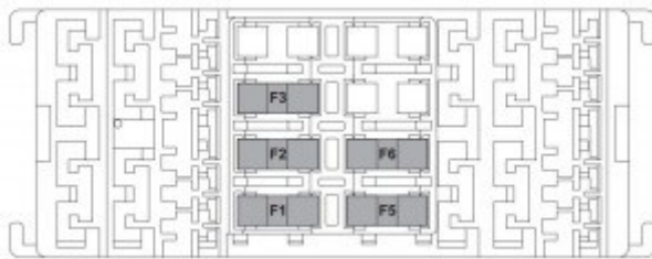
Fiat 500L LIVING – fuse box – luggage
