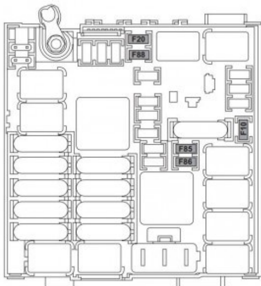
Fiat 500L LIVING – fuse box – engine compartment
