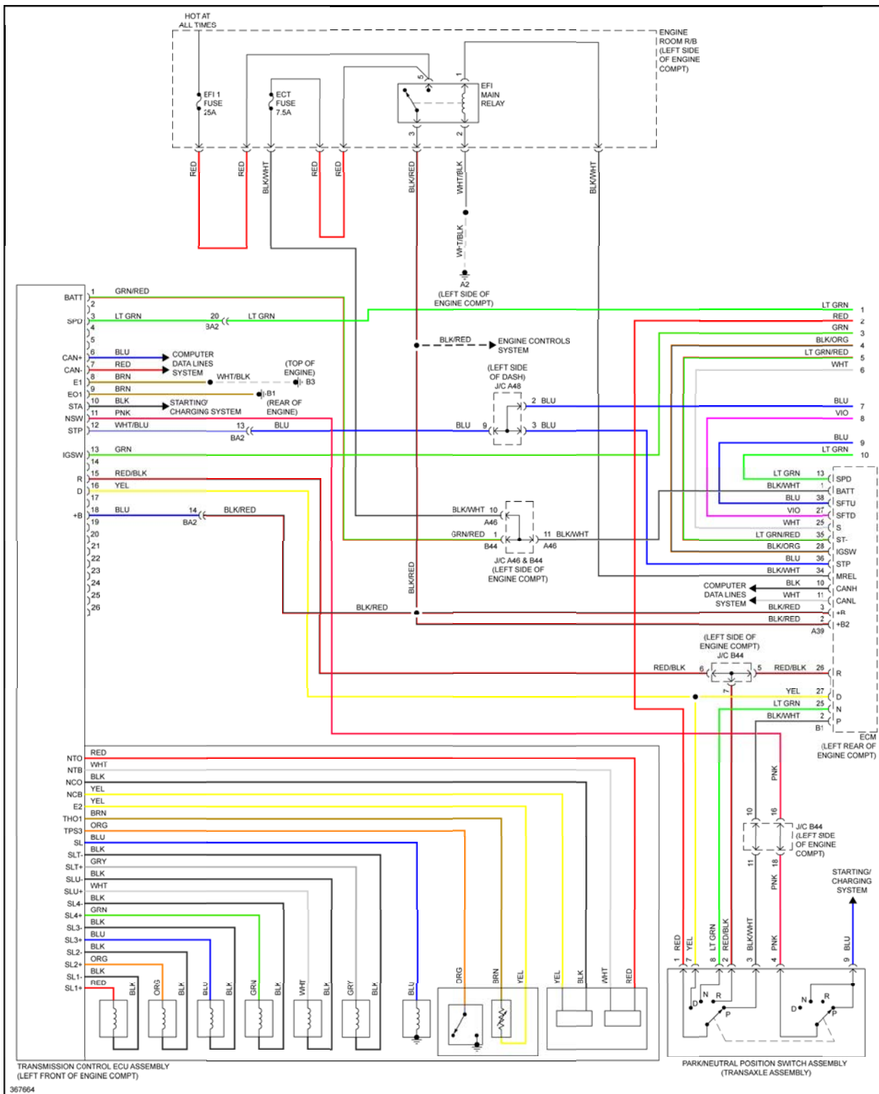
Fig. 114: 3.5L, A/T Circuit (1 of 2)
