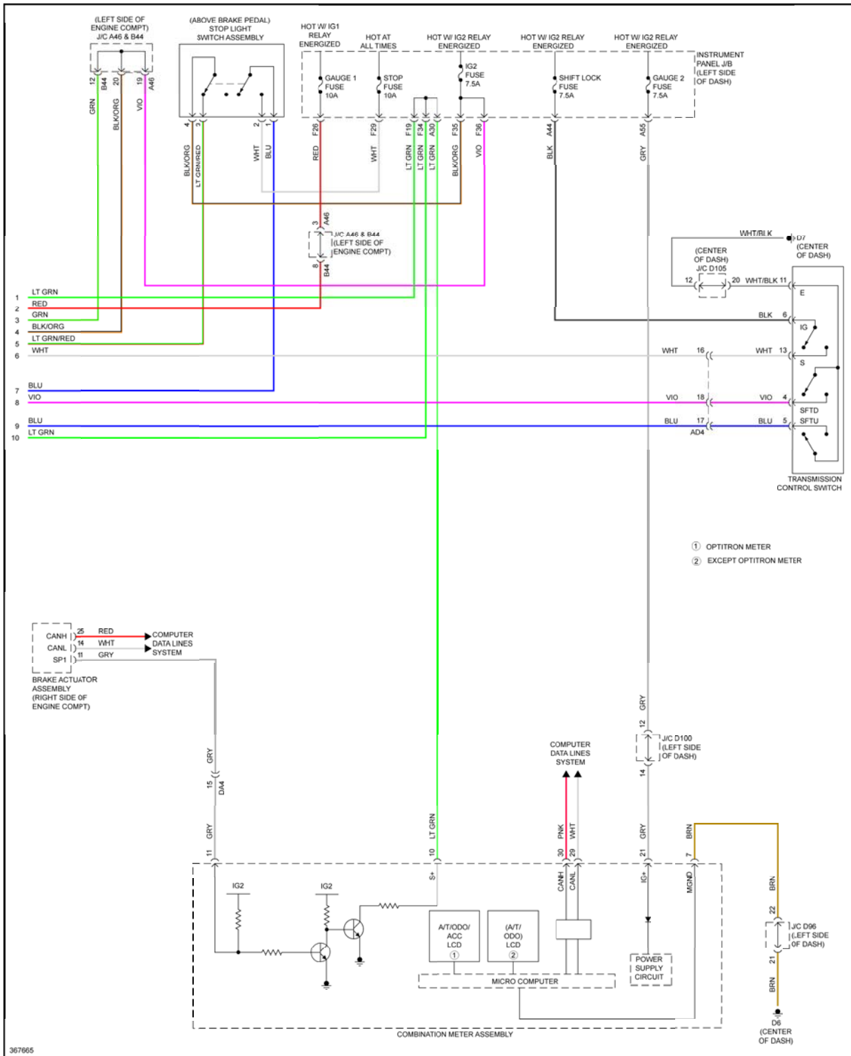
Fig. 115: 3.5L, A/T Circuit (2 of 2)
