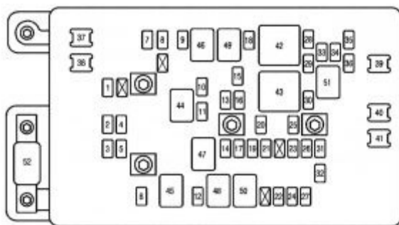
Chevrolet SSR – fuse box diagram – engine
