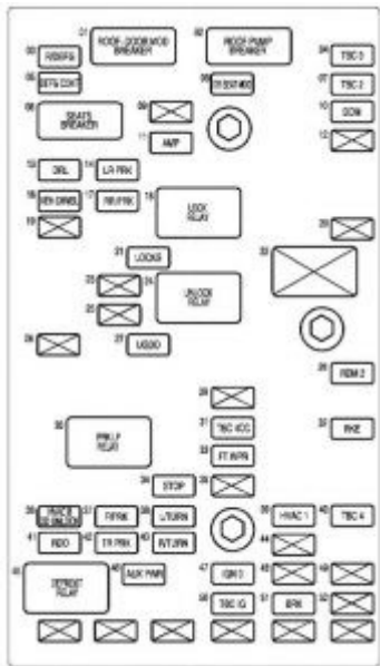
Chevrolet SSR – fuse box diagram – center console
