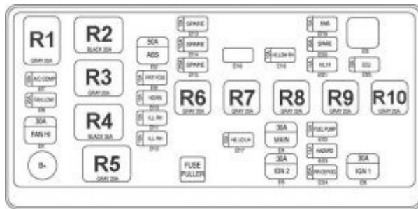
Chevrolet Spark – fuse box diagram – engine
