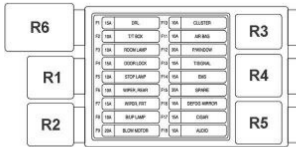
Chevrolet Spark – fuse box diagram – instrument
