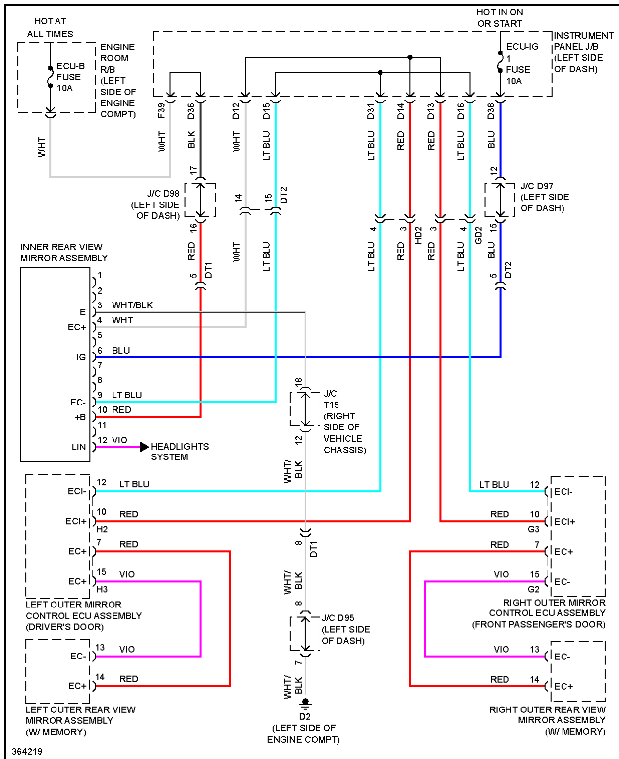
Fig. 80: Electrochromic Mirror Circuit
