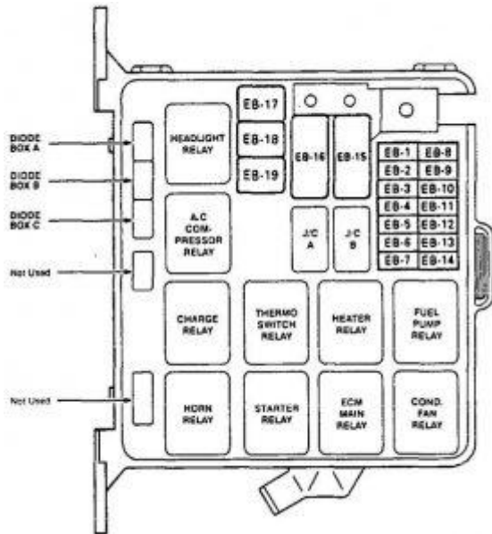
Isuzu Rodeo – fuse box diagram
