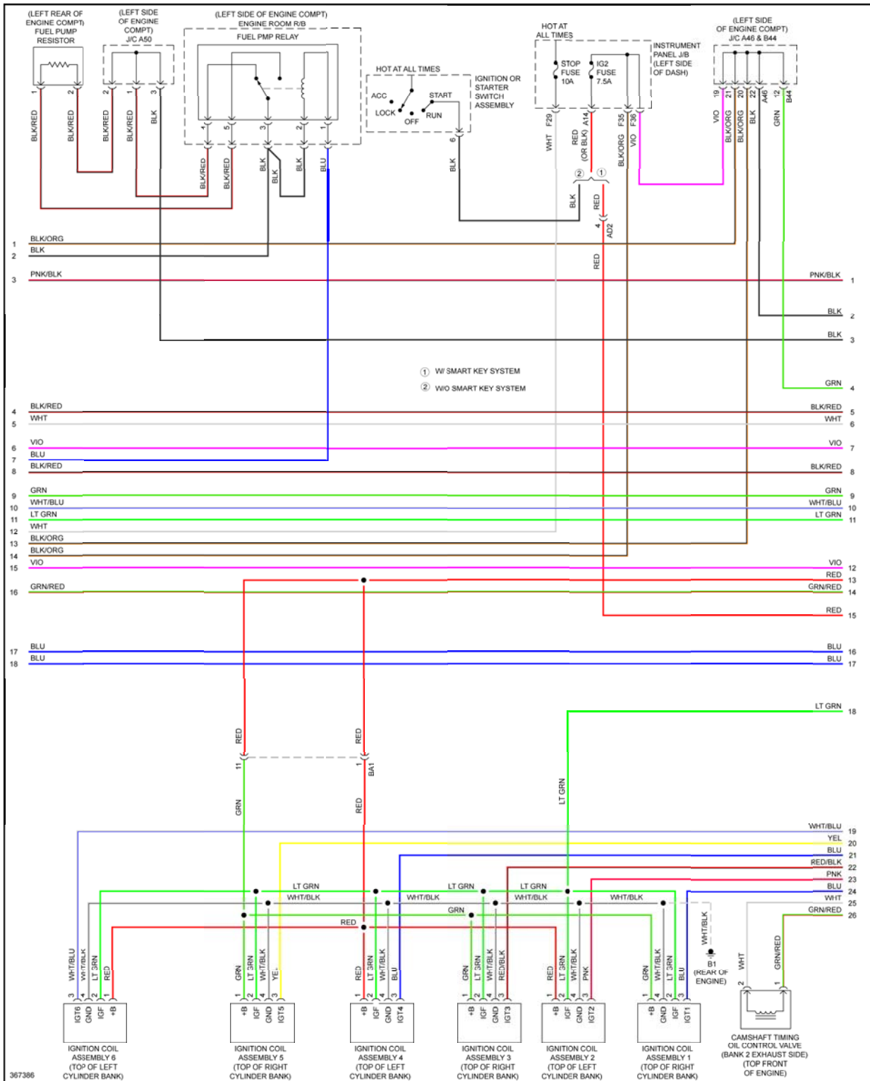
Fig. 34: 3.5L, Engine Performance Circuit (2 of 6)
