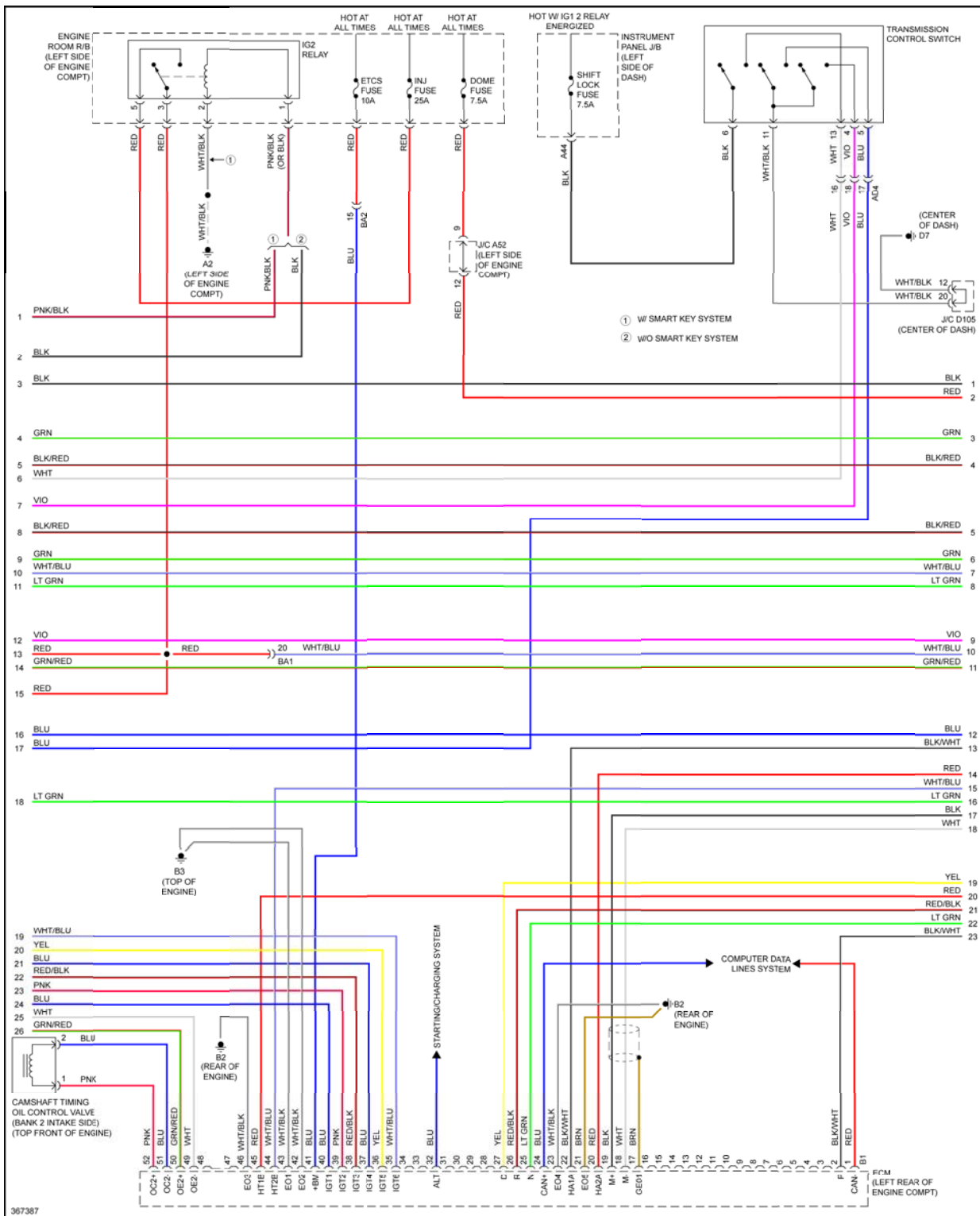
Fig. 35: 3.5L, Engine Performance Circuit (3 of 6)
