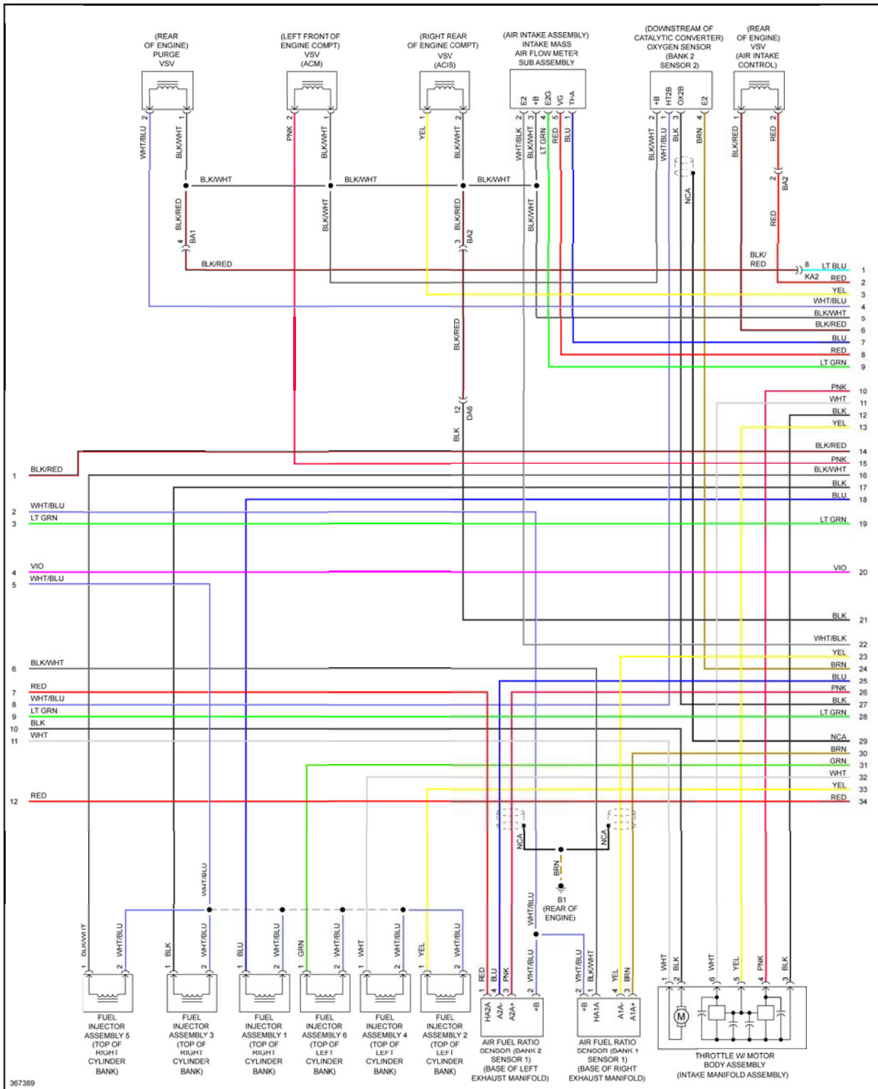
Fig. 37: 3.5L, Engine Performance Circuit (5 of 6)
