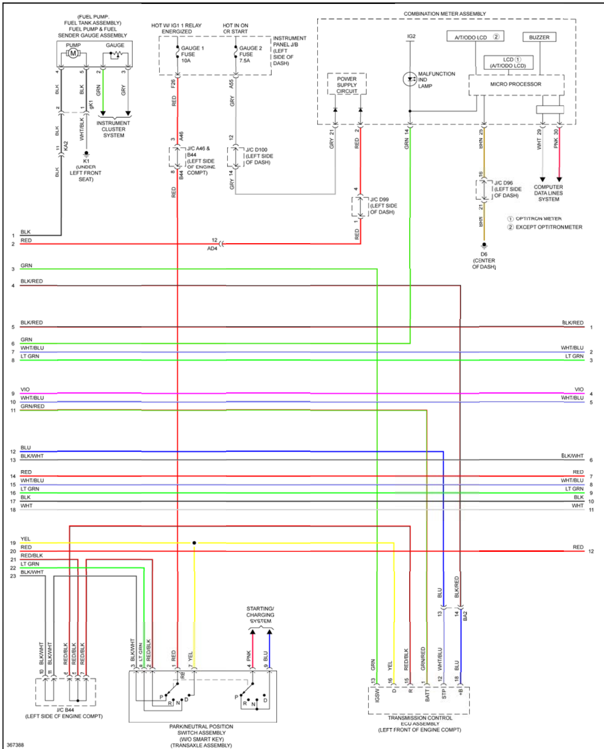
Fig. 36: 3.5L, Engine Performance Circuit (4 of 6)
