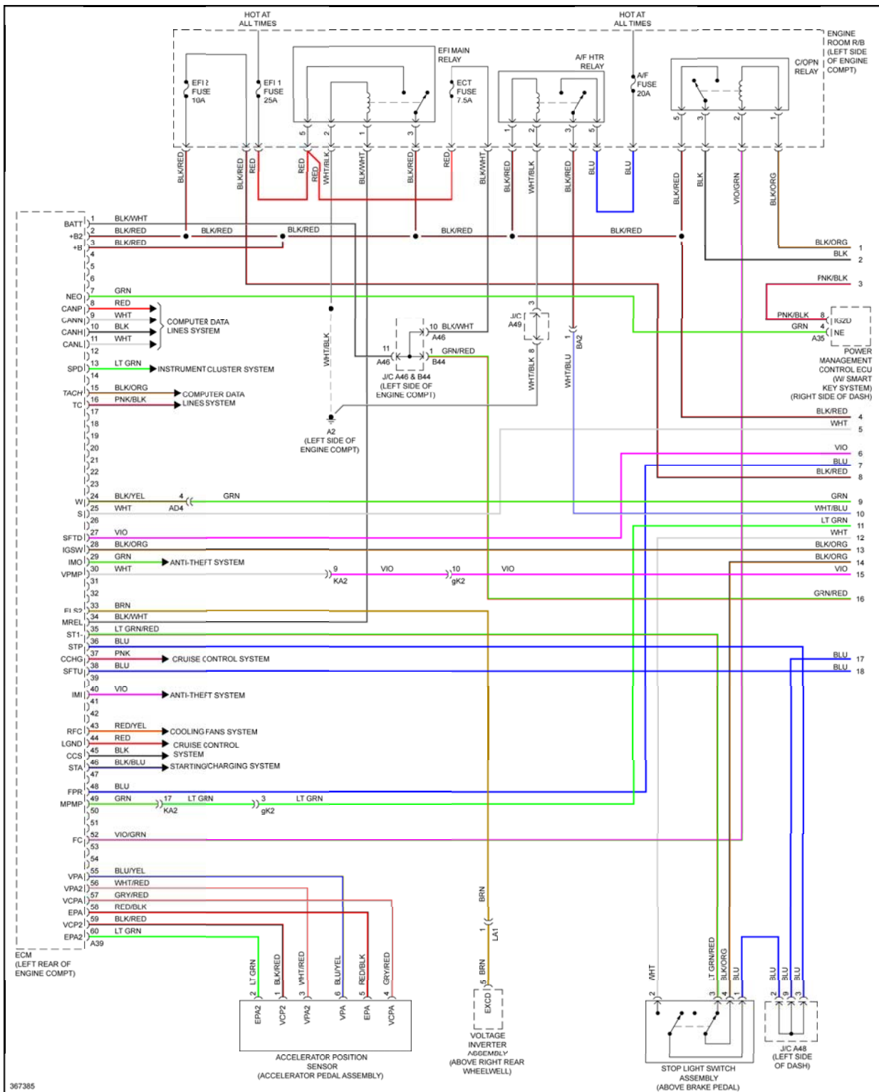
Fig. 33: 3.5L, Engine Performance Circuit (1 of 6)
