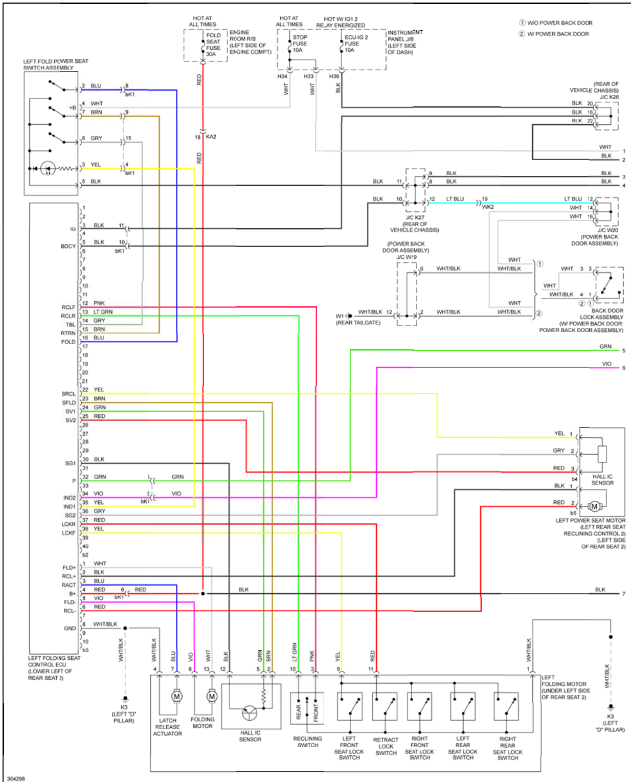
Fig. 87: Third Row Folding Seat Circuit (1 of 2)
