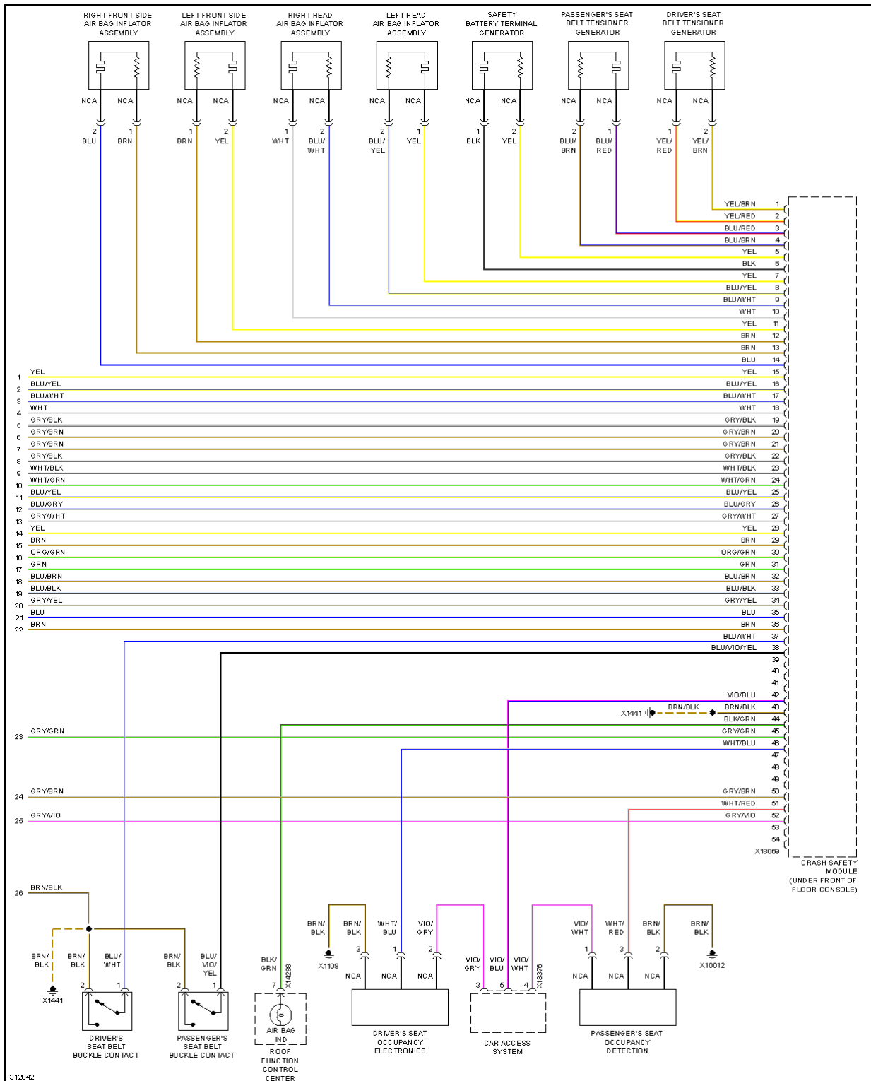
Fig. 122: Supplemental Restraints Circuit (3 of 3)
