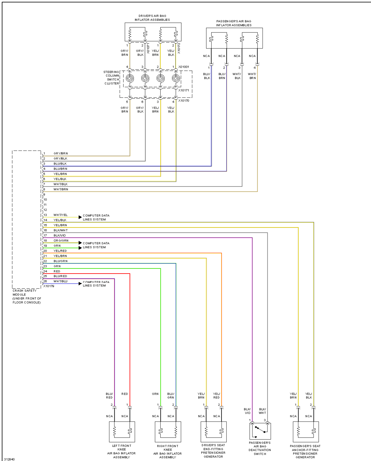
Fig. 120: Supplemental Restraints Circuit (1 of 3)
