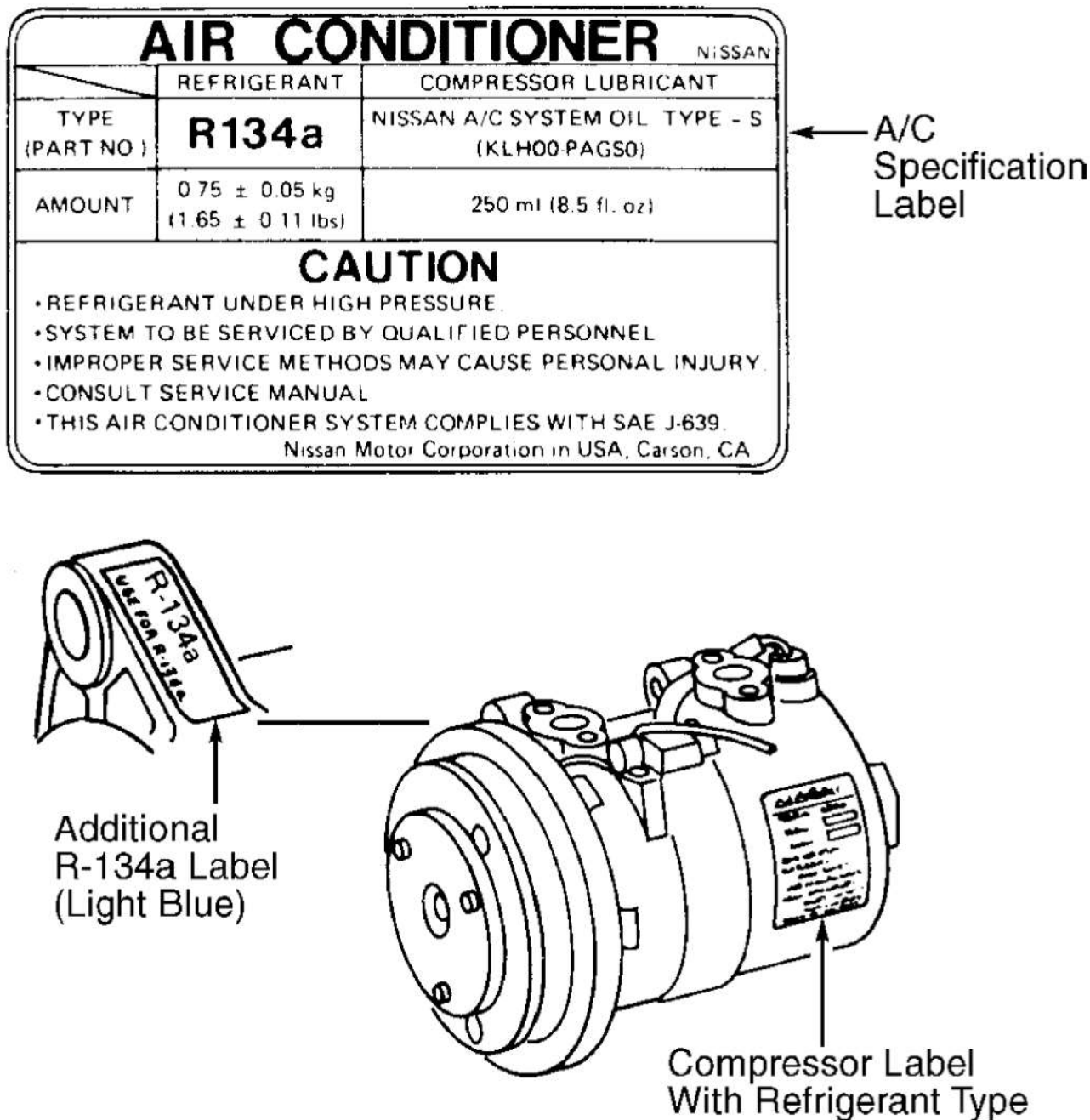
Fig. 2: Underhood A/C Specification Labels (Typical) Courtesy of Nissan Motor Co., U.S.A.
