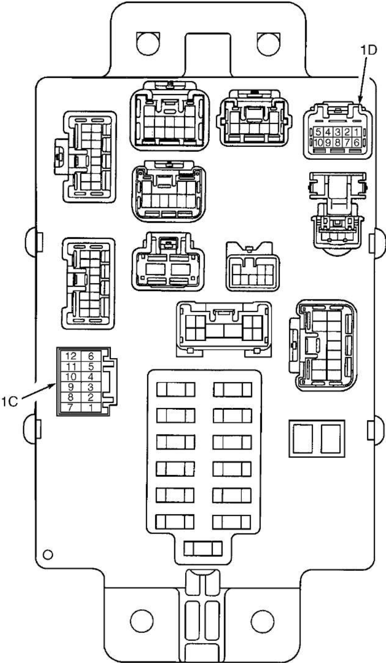
Fig. 23: Identifying Instrument Panel Junction Box Harness Connector 1C & 1D Terminals (RAV4) Courtesy of TOYOTA MOTOR SALES, U.S.A., INC.
