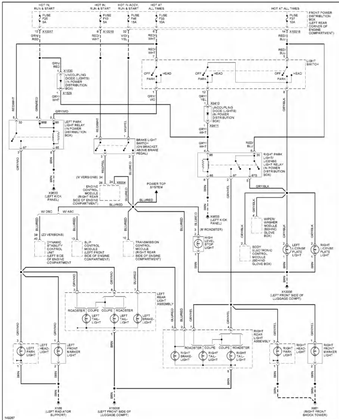
Fig. 28: Park, Stop, Tail & License Plate Lamps Circuit, Canada
