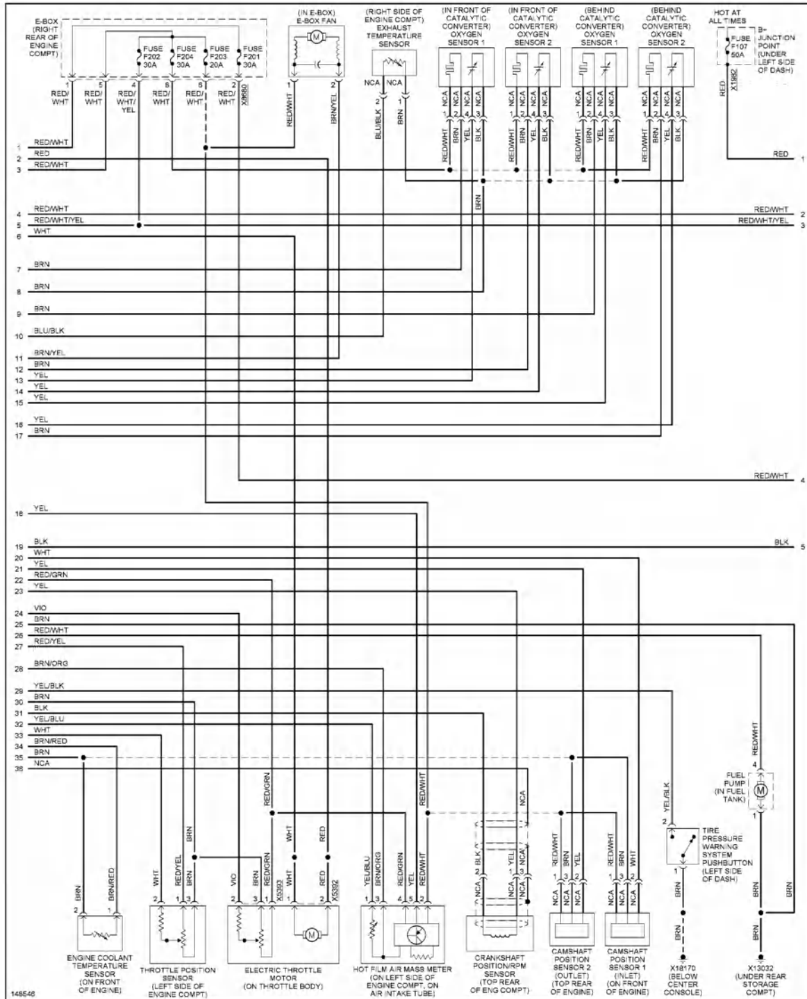
Fig. 24: 3.3L Engine Performance Circuit (2 of 4)
