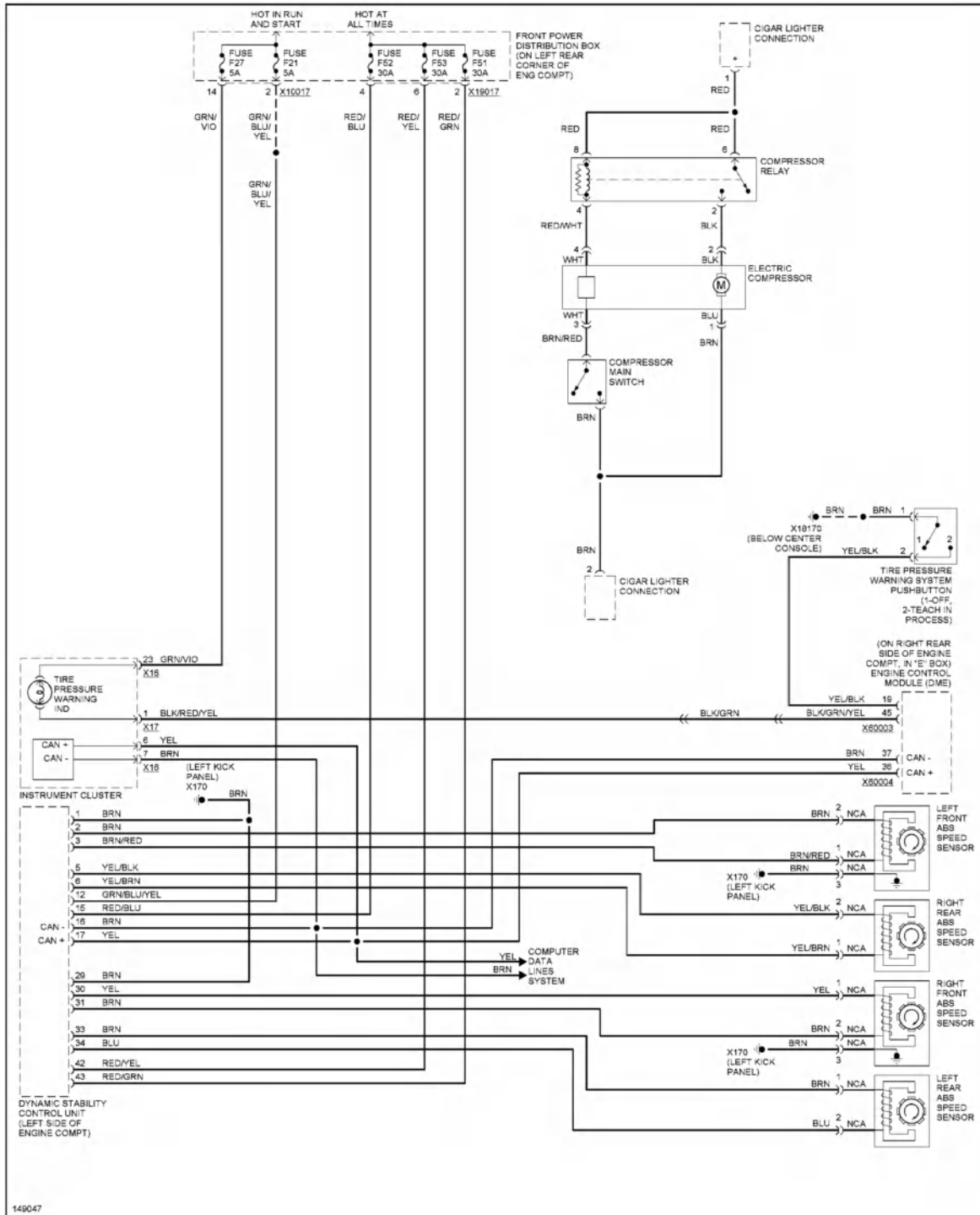
Fig. 72: Tire Pressure Monitoring/Inflation Circuit
