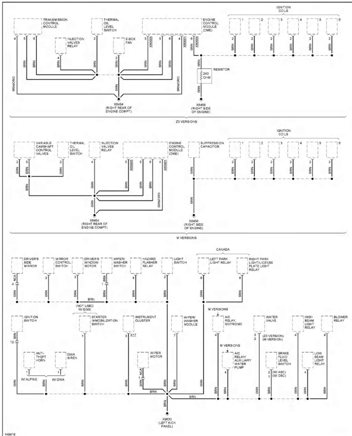
Fig. 32: Ground Distribution Circuit (2 of 4)
