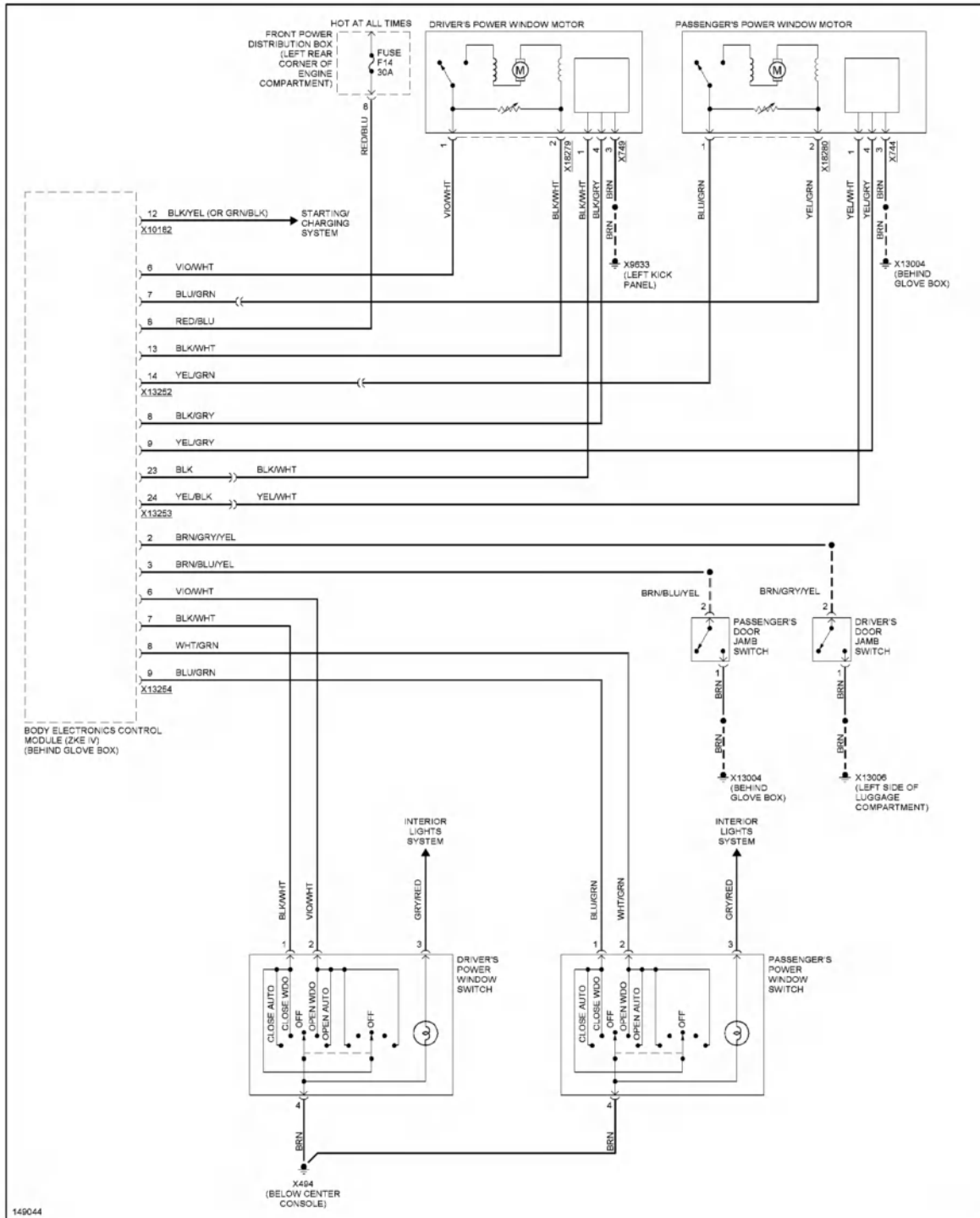
Fig. 61: Power Windows Circuit
