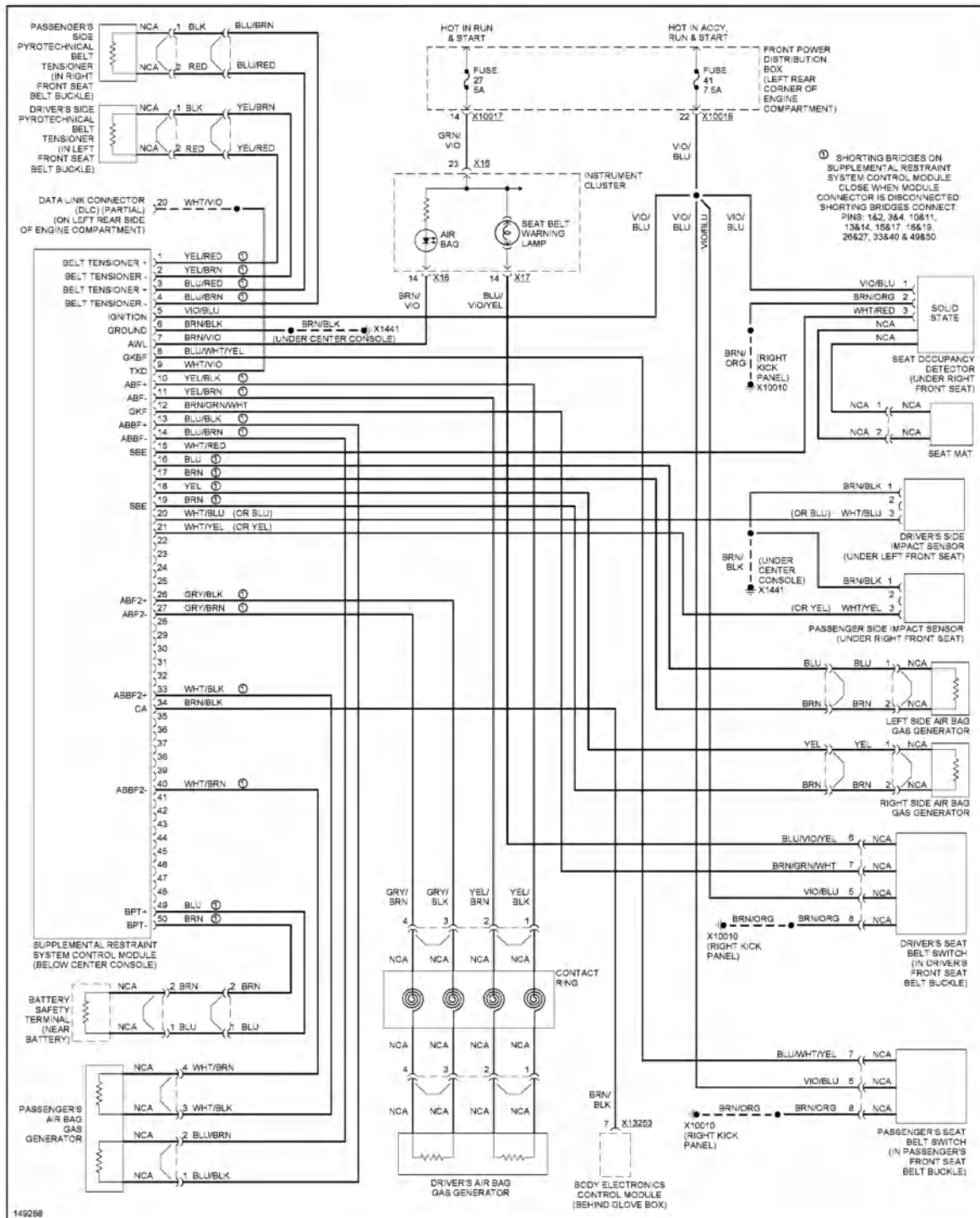
Fig. 69: Supplemental Restraints Circuit
