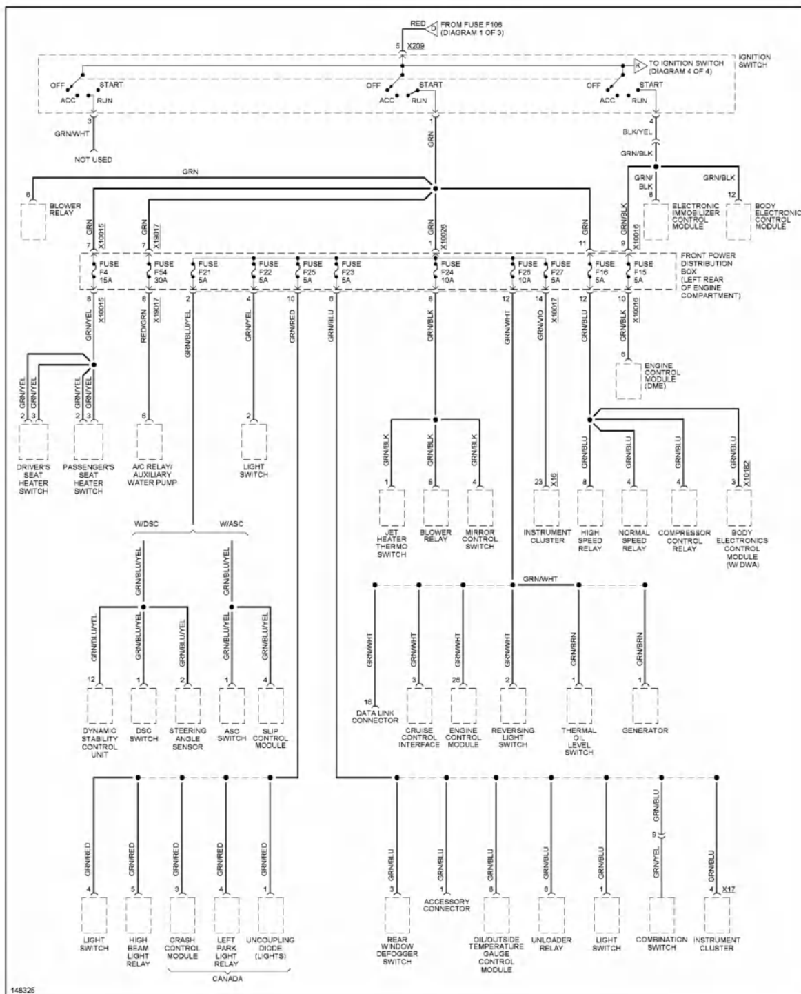
Fig. 45: Power Distribution Circuit, M-Versions (3 of 4)
