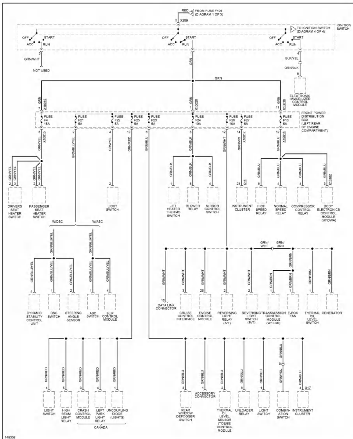
Fig. 49: Power Distribution Circuit, Z3 Versions (3 of 4)
