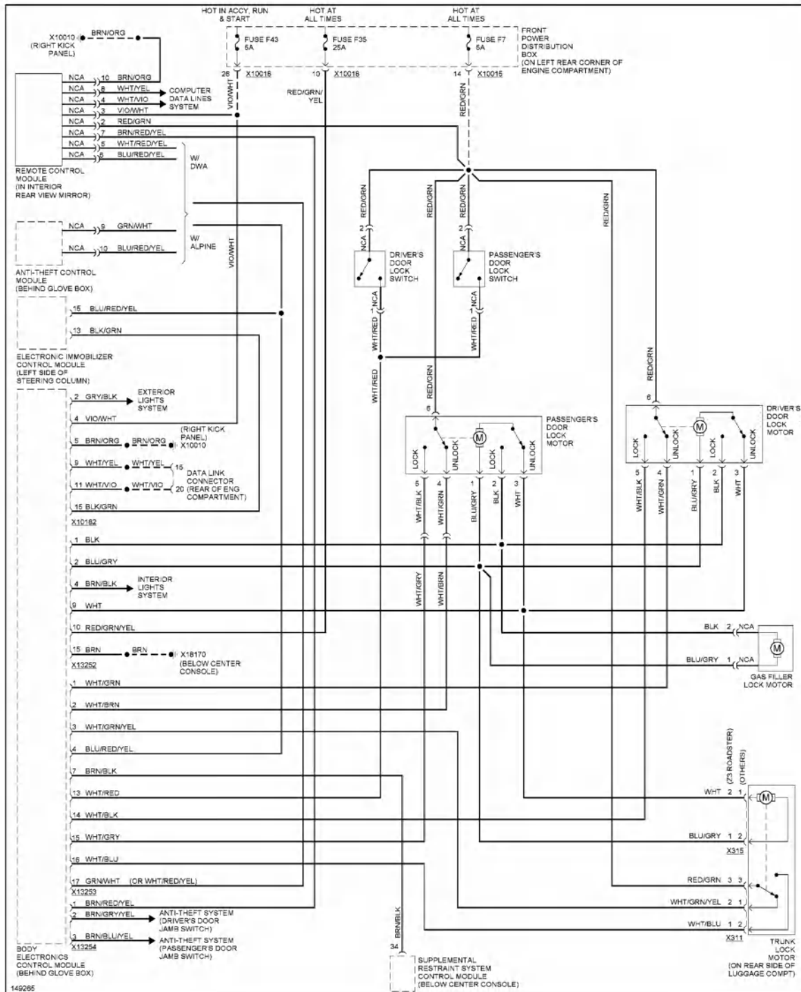
Fig. 51: Power Door Locks Circuit, Except M Version Coupe
