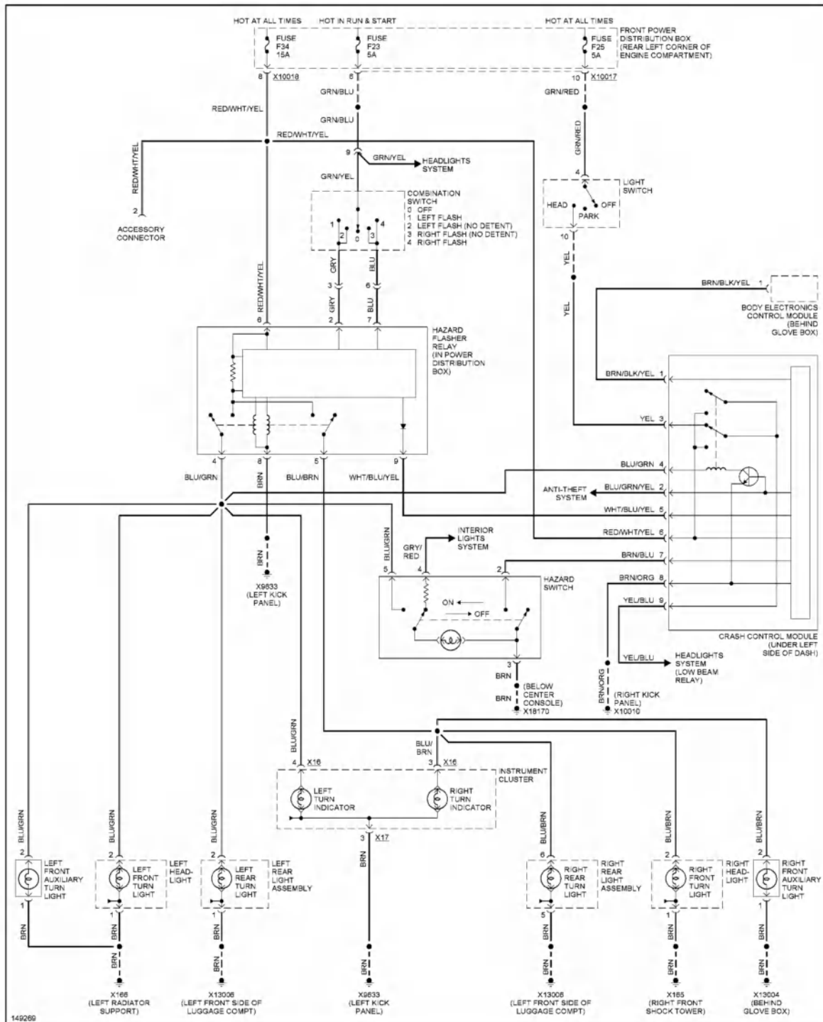
Fig. 30: Turn & Hazard Lamps Circuit
