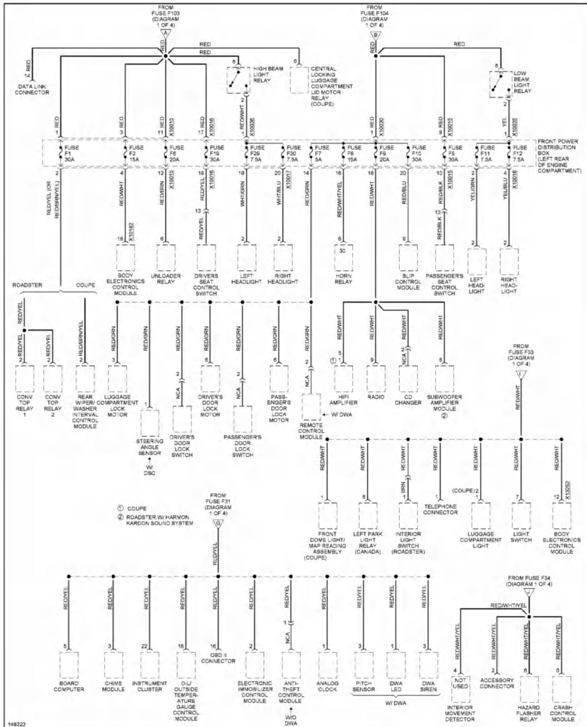
Fig. 44: Power Distribution Circuit, M-Versions (2 of 4)
