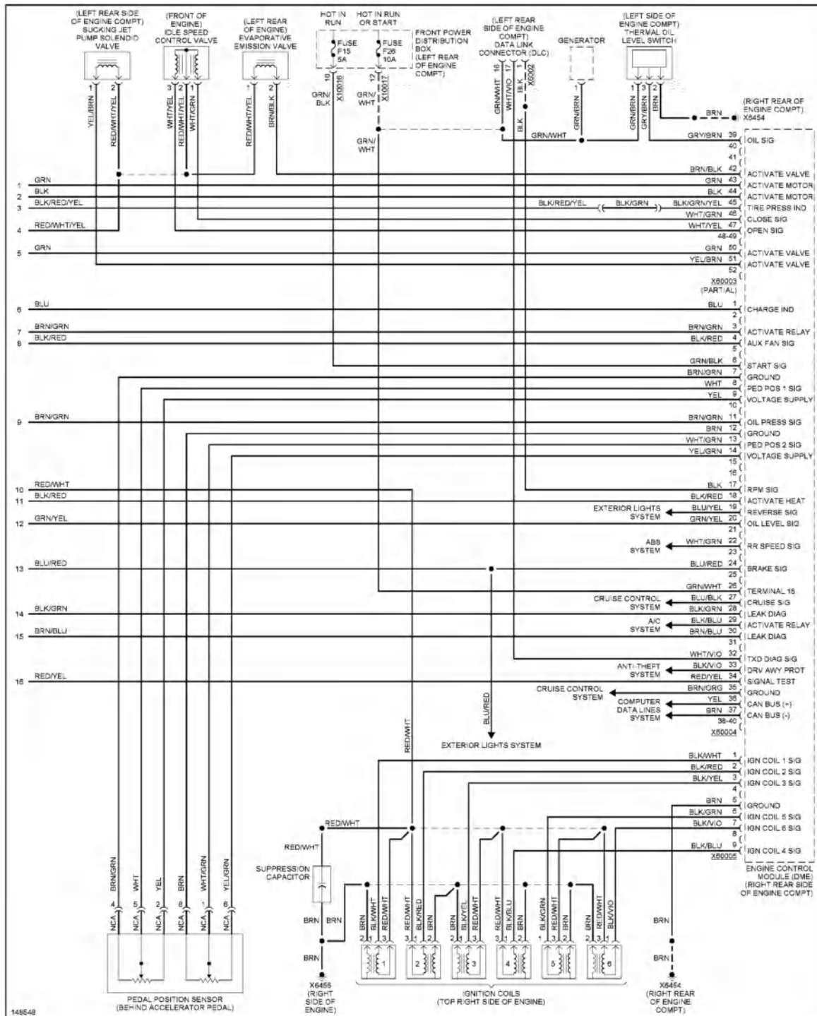
Fig. 26: 3.3L Engine Performance Circuit (4 of 4)
