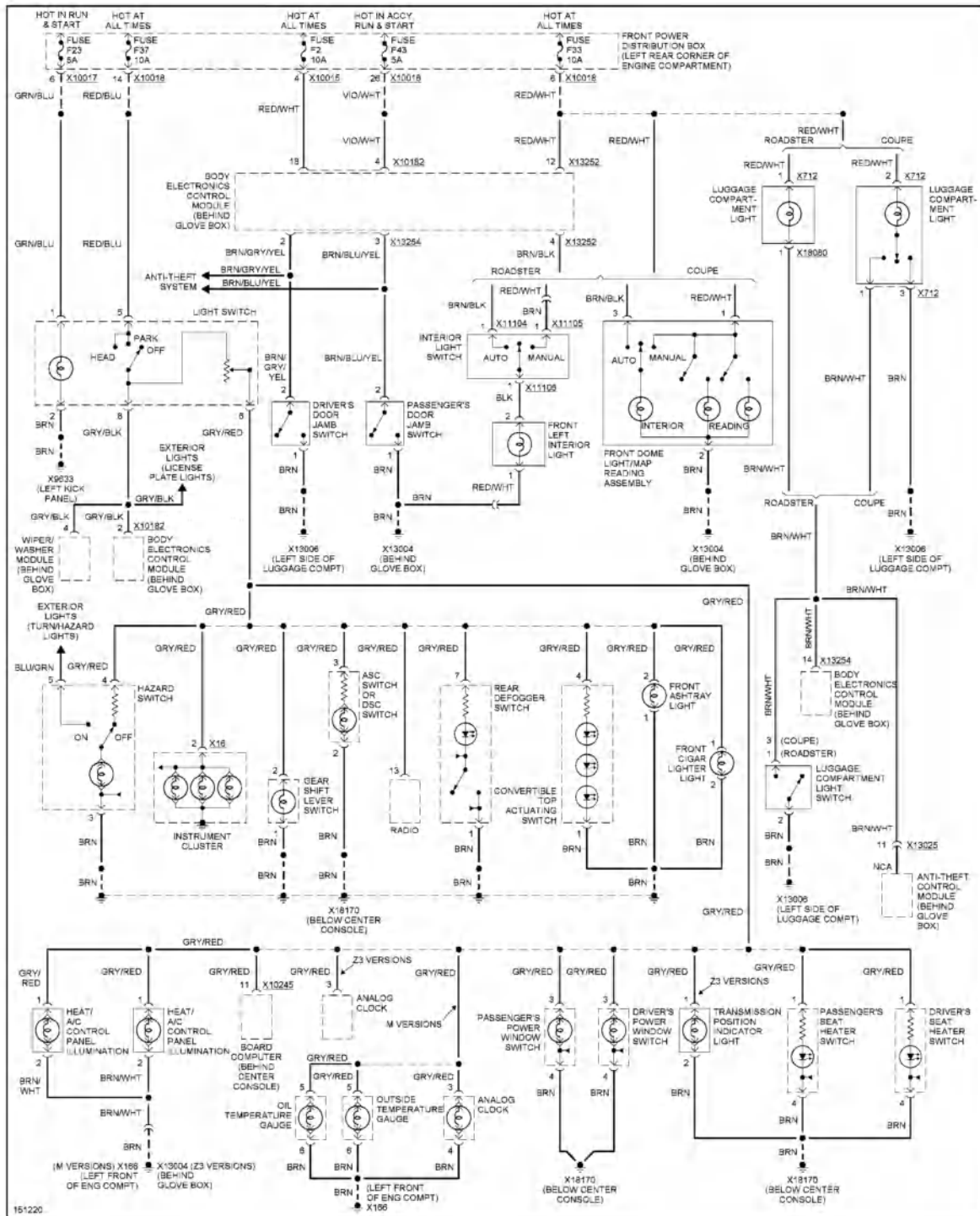
Fig. 42: Interior Lights Circuit
