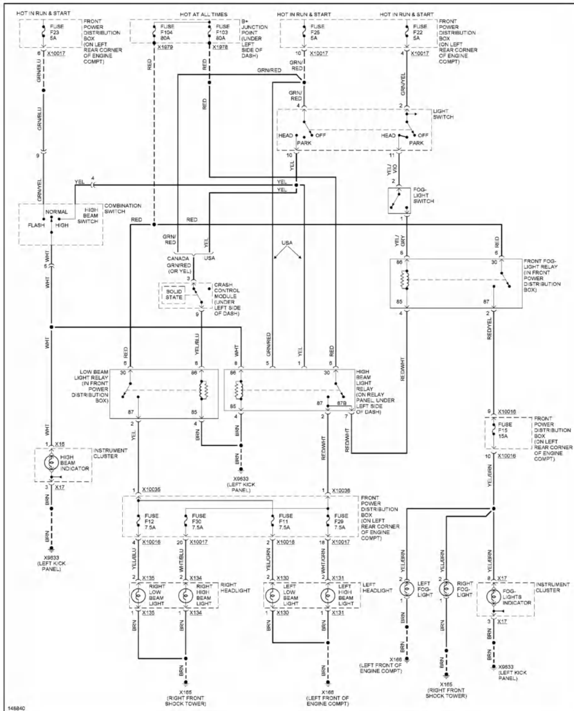
Fig. 35: Headlights Circuit
