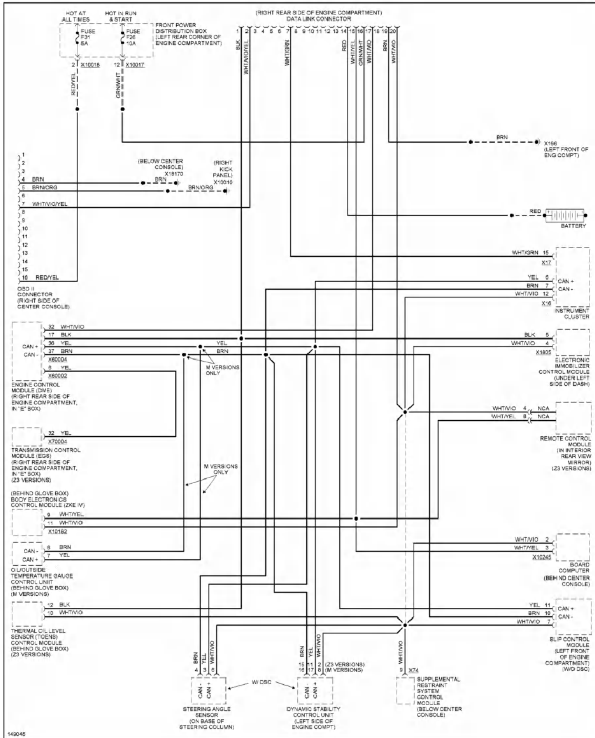
Fig. 10: Computer Data Lines Circuit
