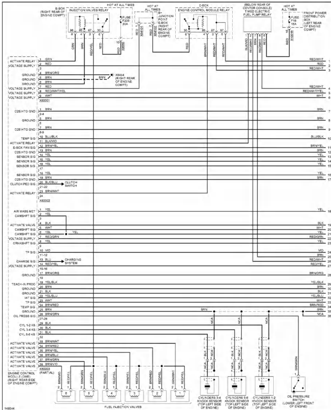
Fig. 23: 3.3L Engine Performance Circuit (1 of 4)
