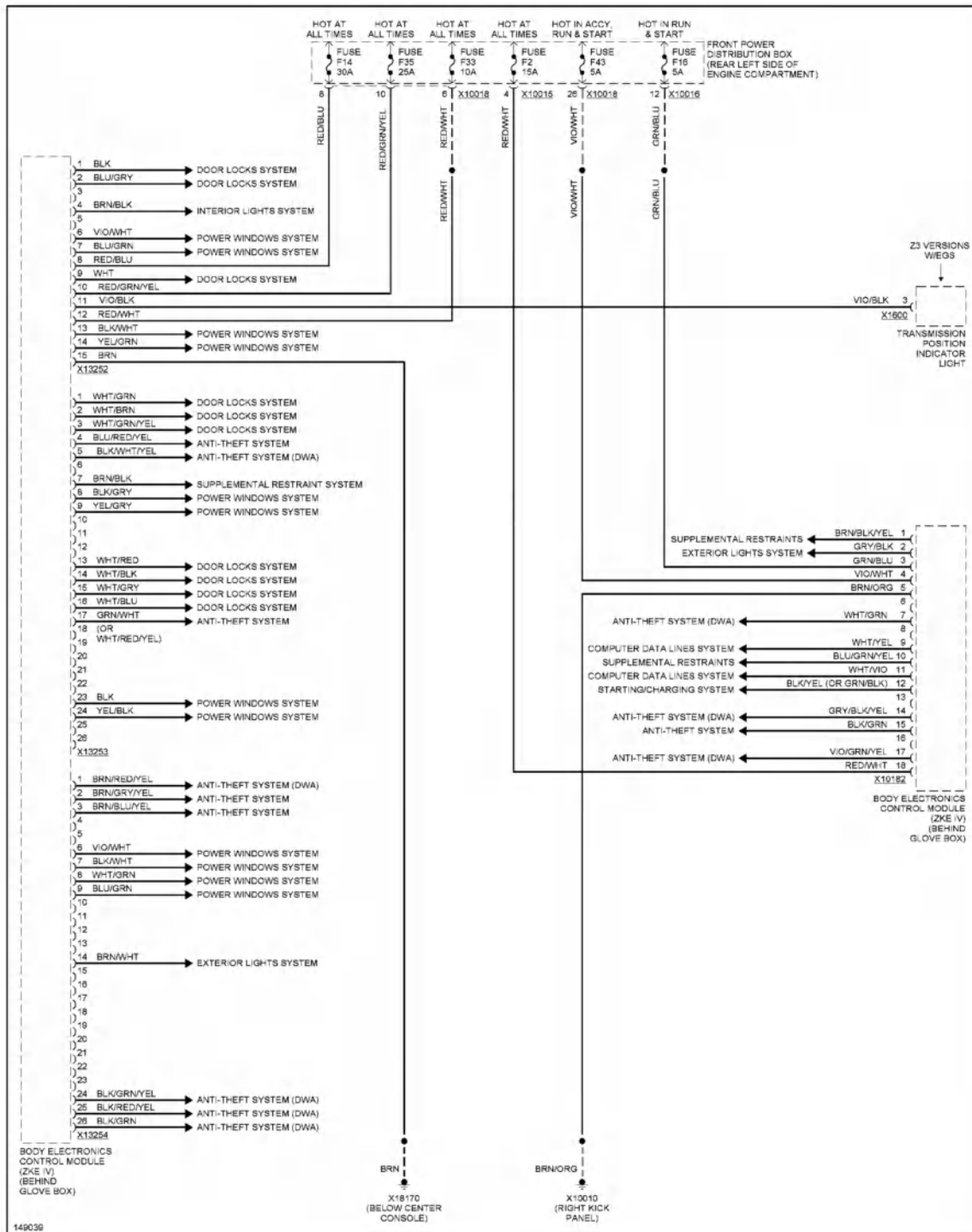
Fig. 9: Body Control Modules Circuit COMPUTER DATA LINES
