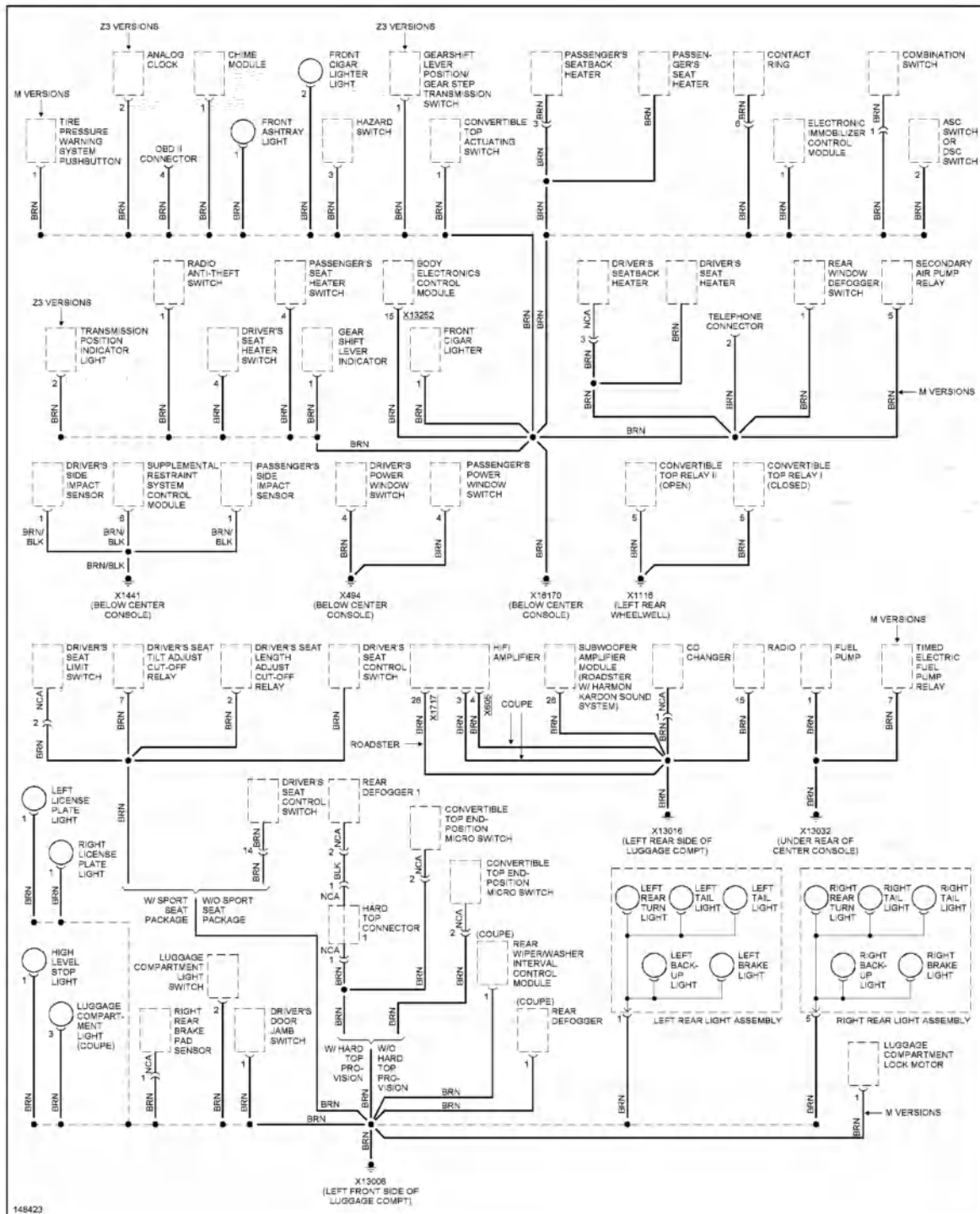
Fig. 34: Ground Distribution Circuit (4 of 4)
