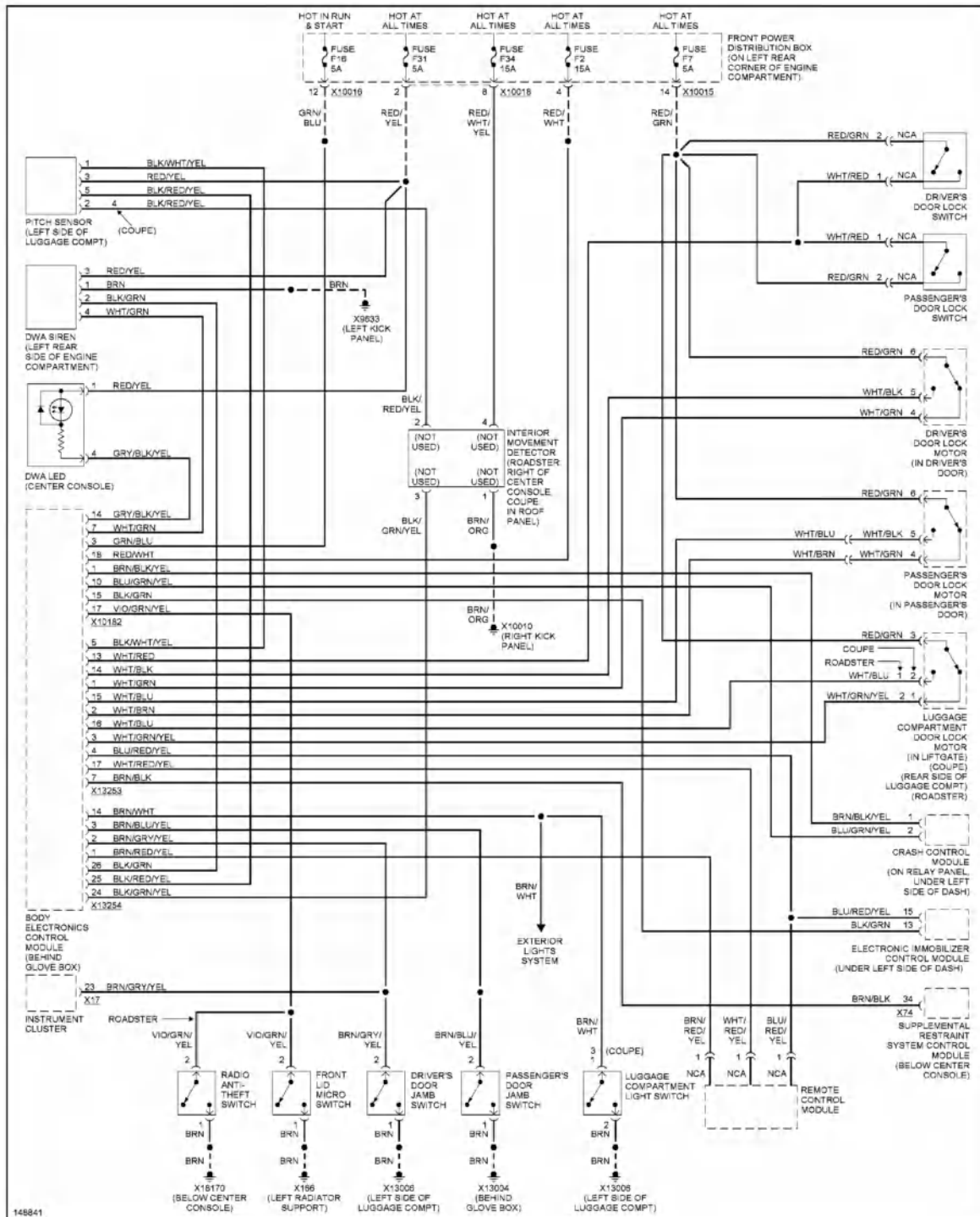
Fig. 8: Forced Entry Circuit, DWA
