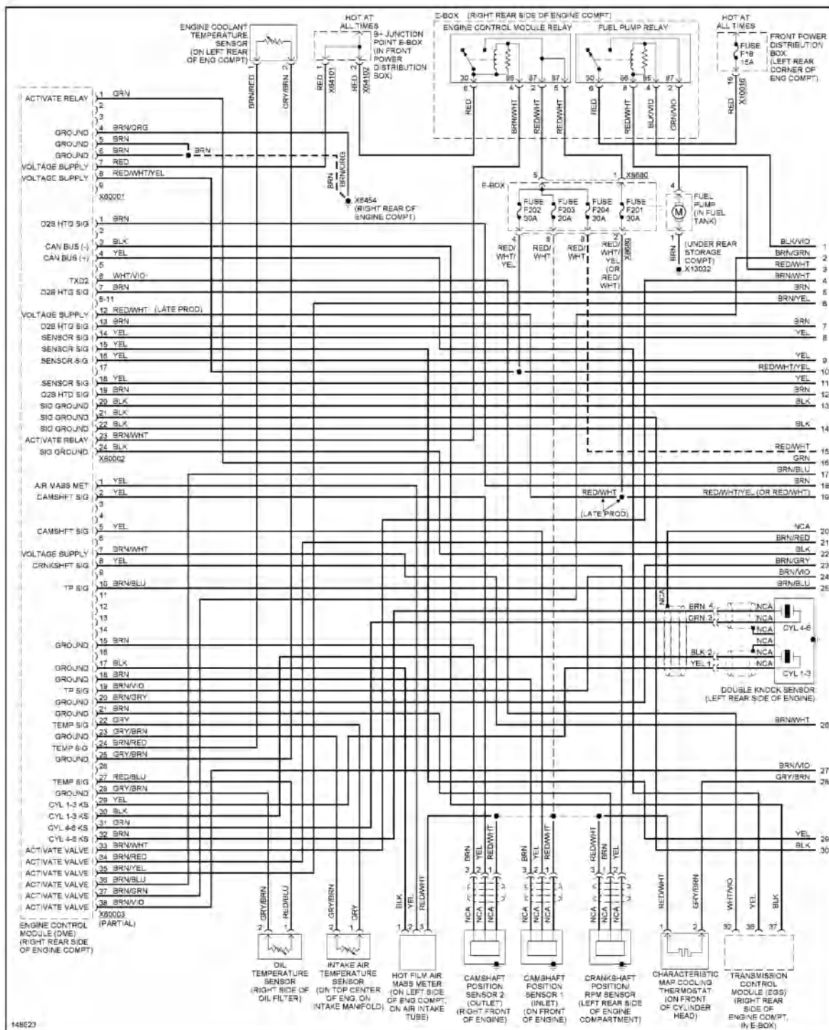
Fig. 17: 2.5L, Engine Performance Circuit (1 of 3)
