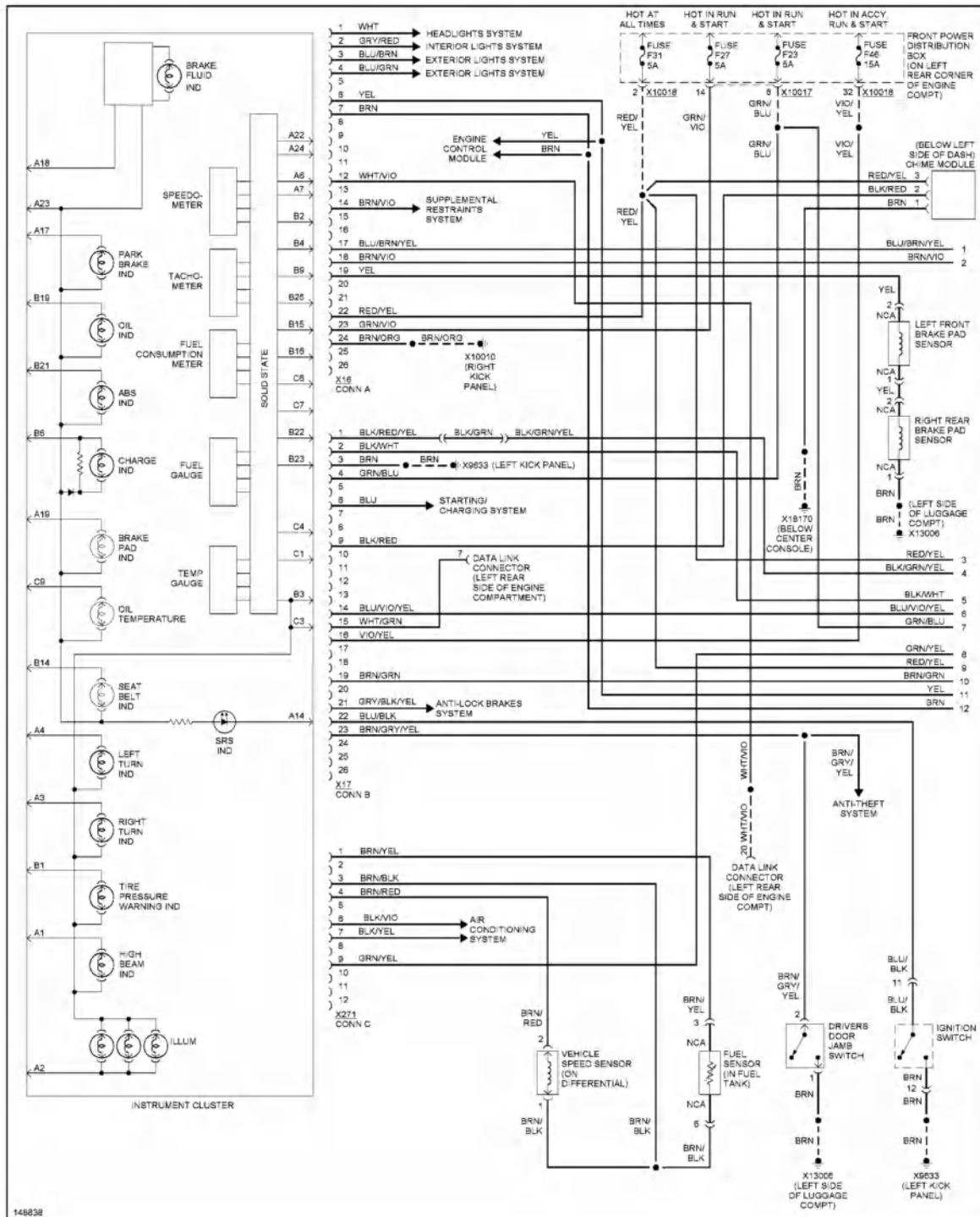
Fig. 37: Instrument Cluster Circuit, M-Versions (1 of 2)
