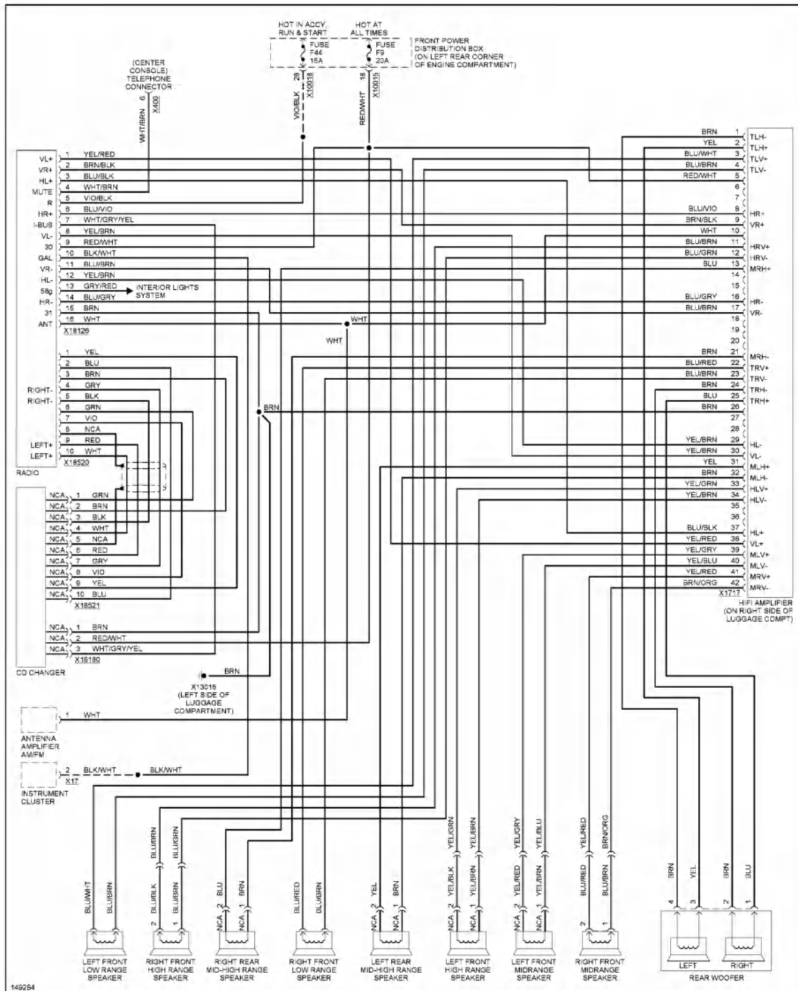
Fig. 64: Radio Circuit, Roadster W/O Harman Kardon
