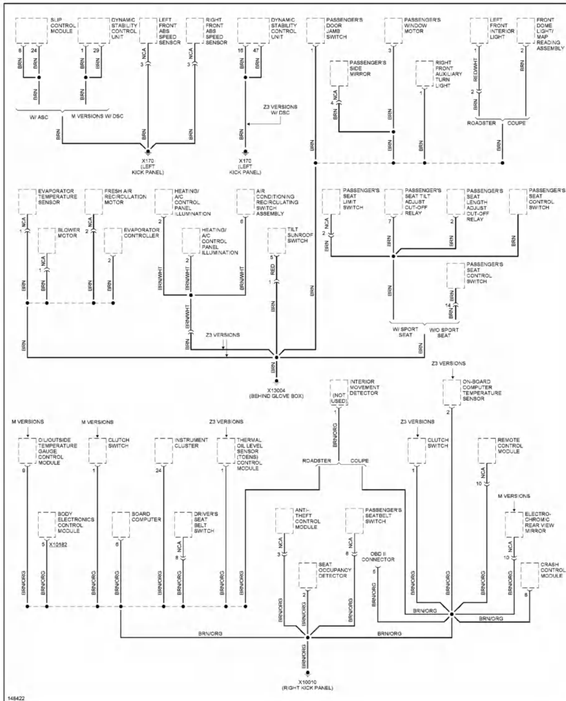
Fig. 33: Ground Distribution Circuit (3 of 4)
