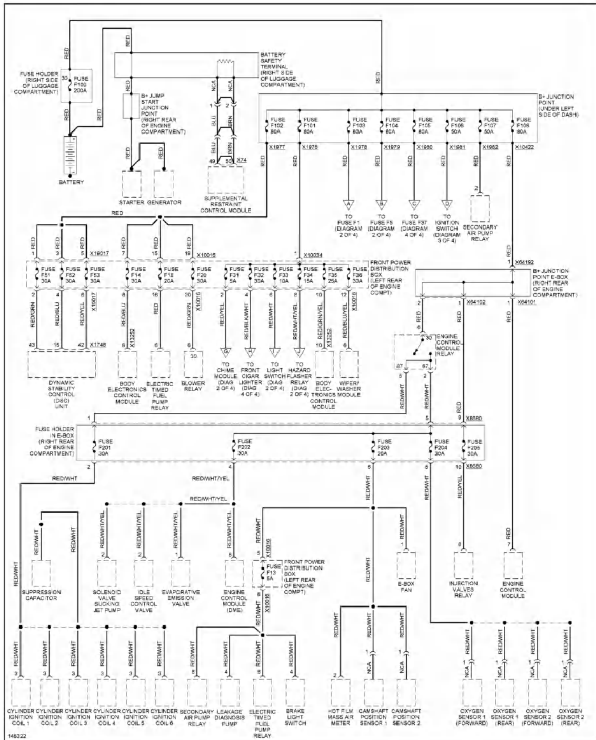
Fig. 43: Power Distribution Circuit, M-Versions (1 of 4)
