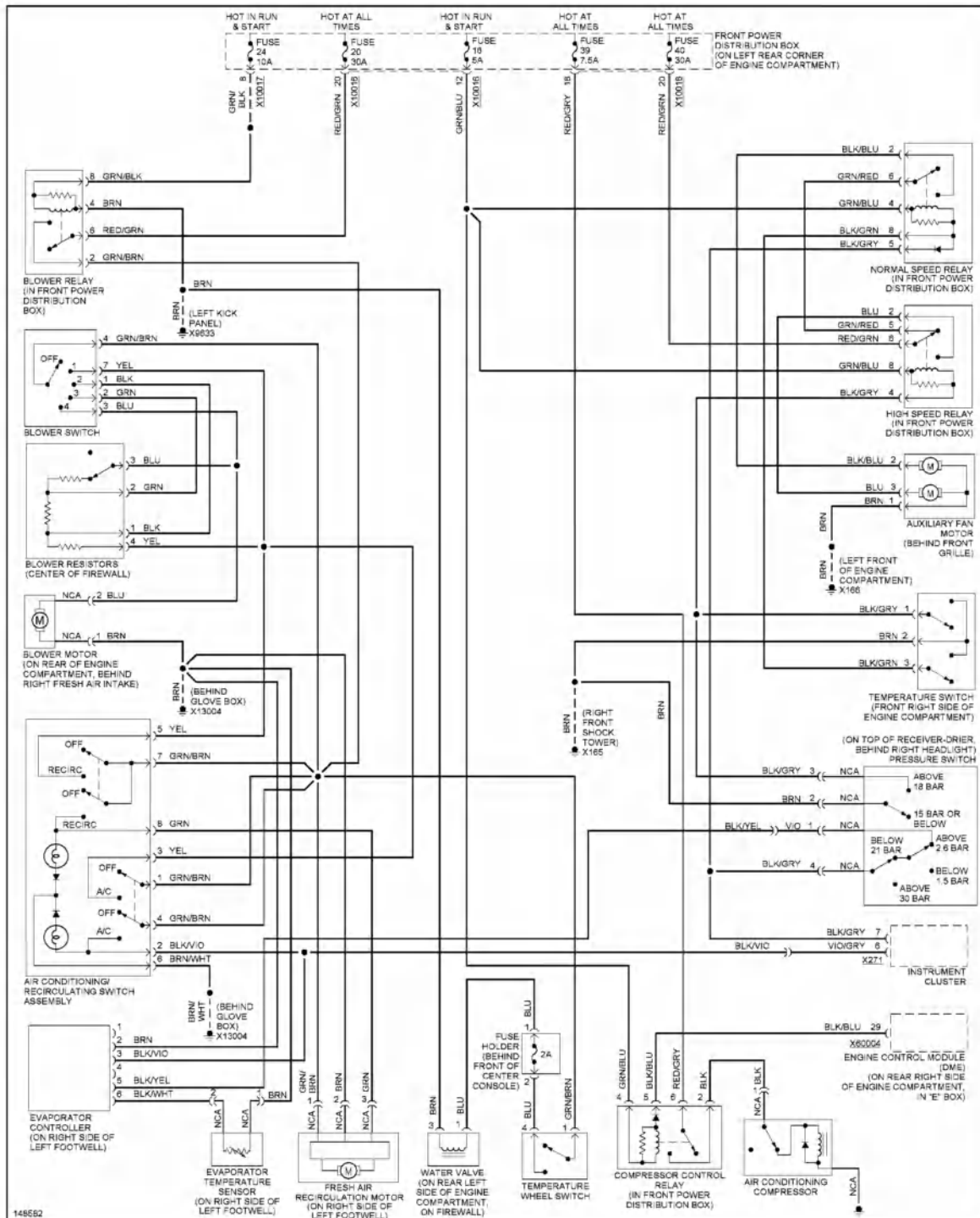
Fig. 2: Manual A/C Circuit, Z3 Versions
