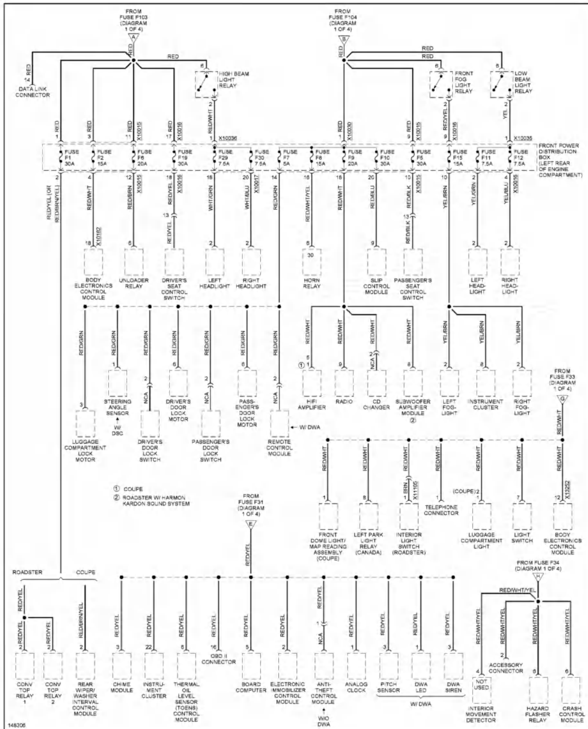
Fig. 48: Power Distribution Circuit, Z3 Versions (2 of 4)
