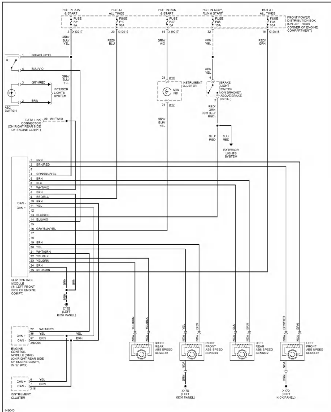
Fig. 5: Anti-lock Brakes Circuit, W/ Slip Control
