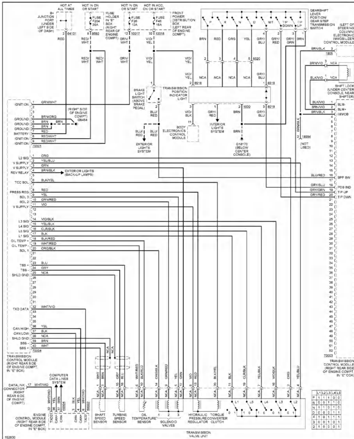
Fig. 70: A/T Circuit WARNING SYSTEMS
