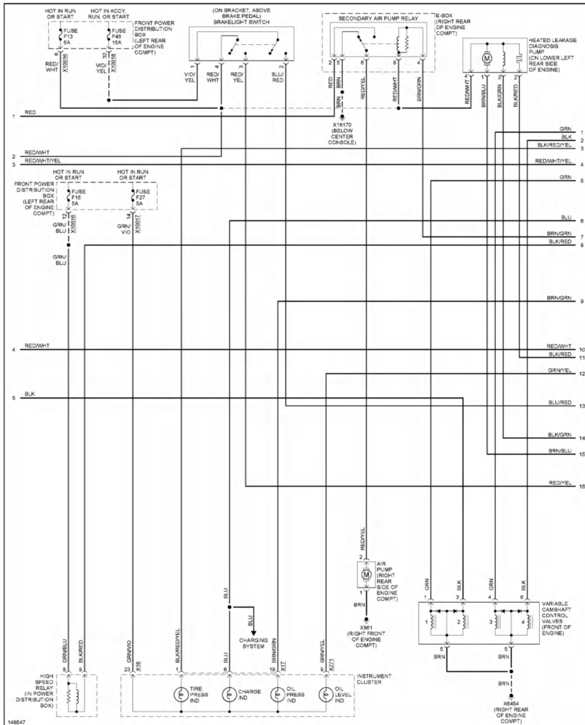
Fig. 25: 3.3L, Engine Performance Circuit (3 of 4)
