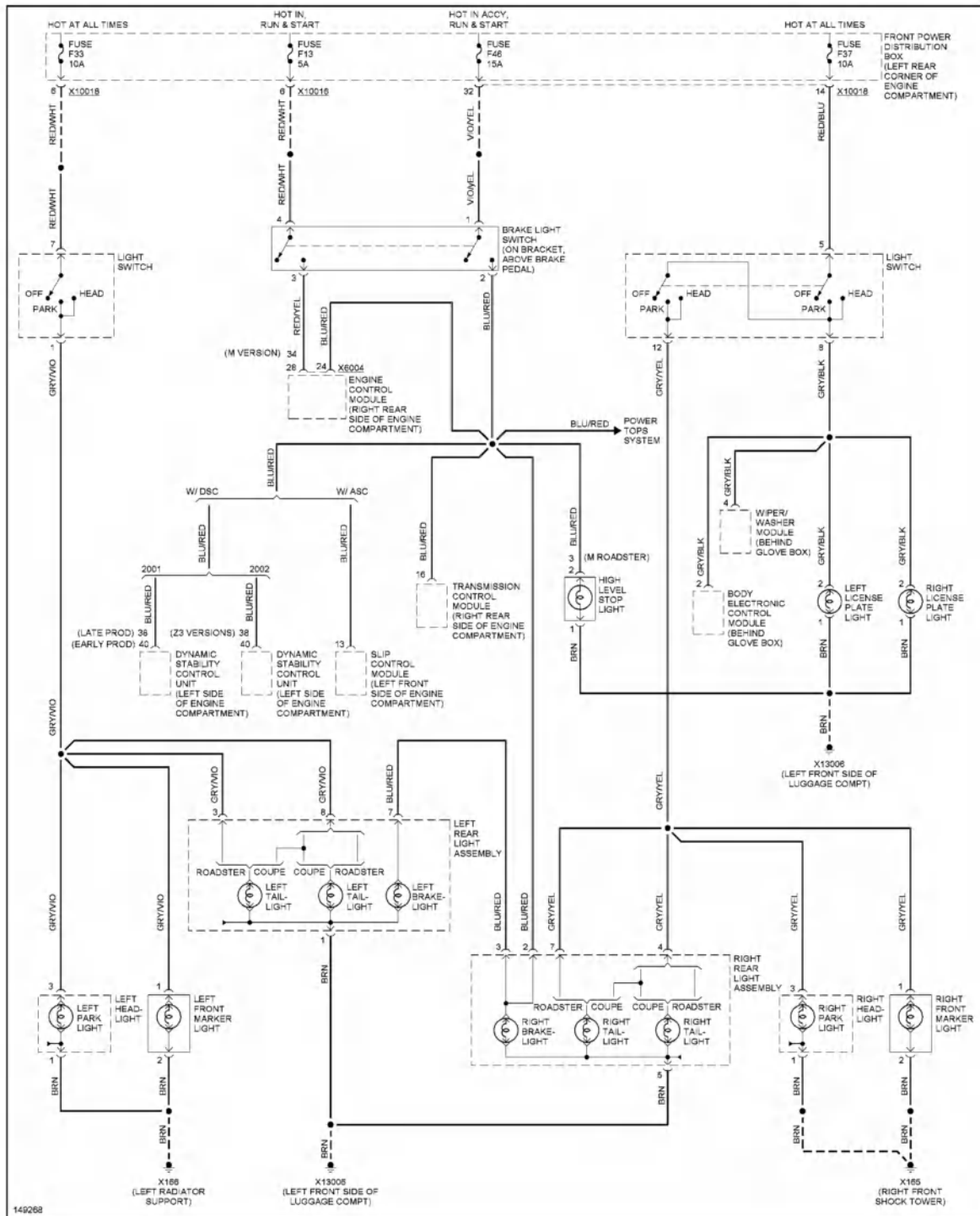
Fig. 29: Park, Stop, Tail & License Plate Lamps Circuit, USA
