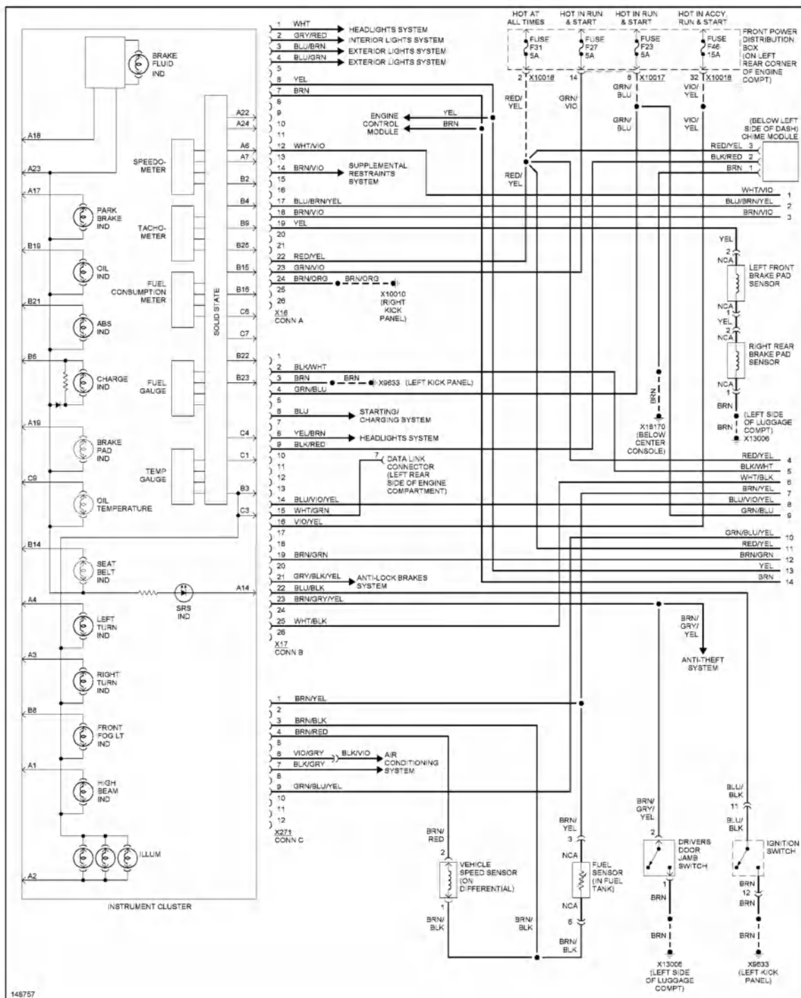
Fig. 39: Instrument Cluster Circuit, Z3 Versions (1 of 2)
