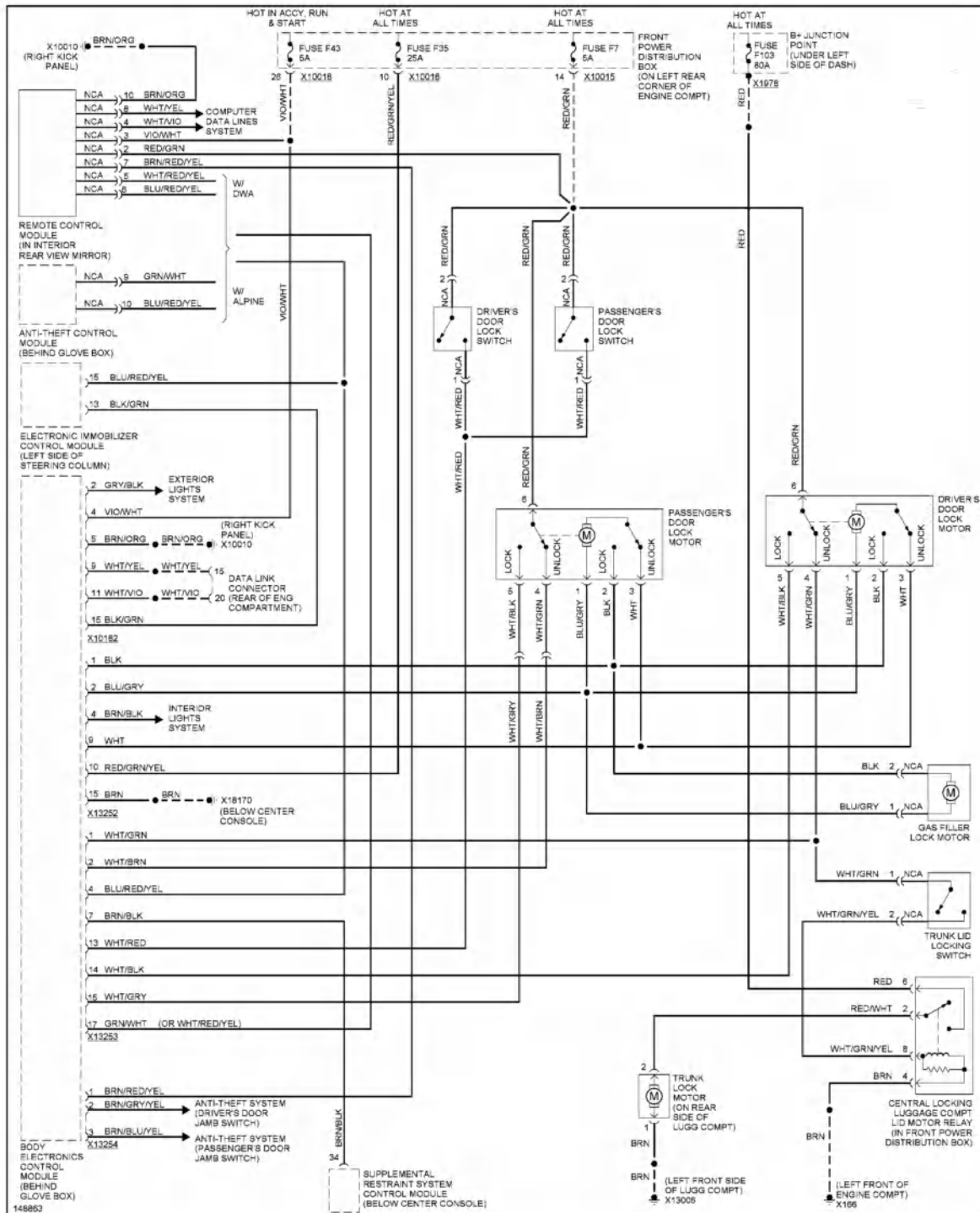
Fig. 52: Power Door Locks Circuit, M Version Coupe
