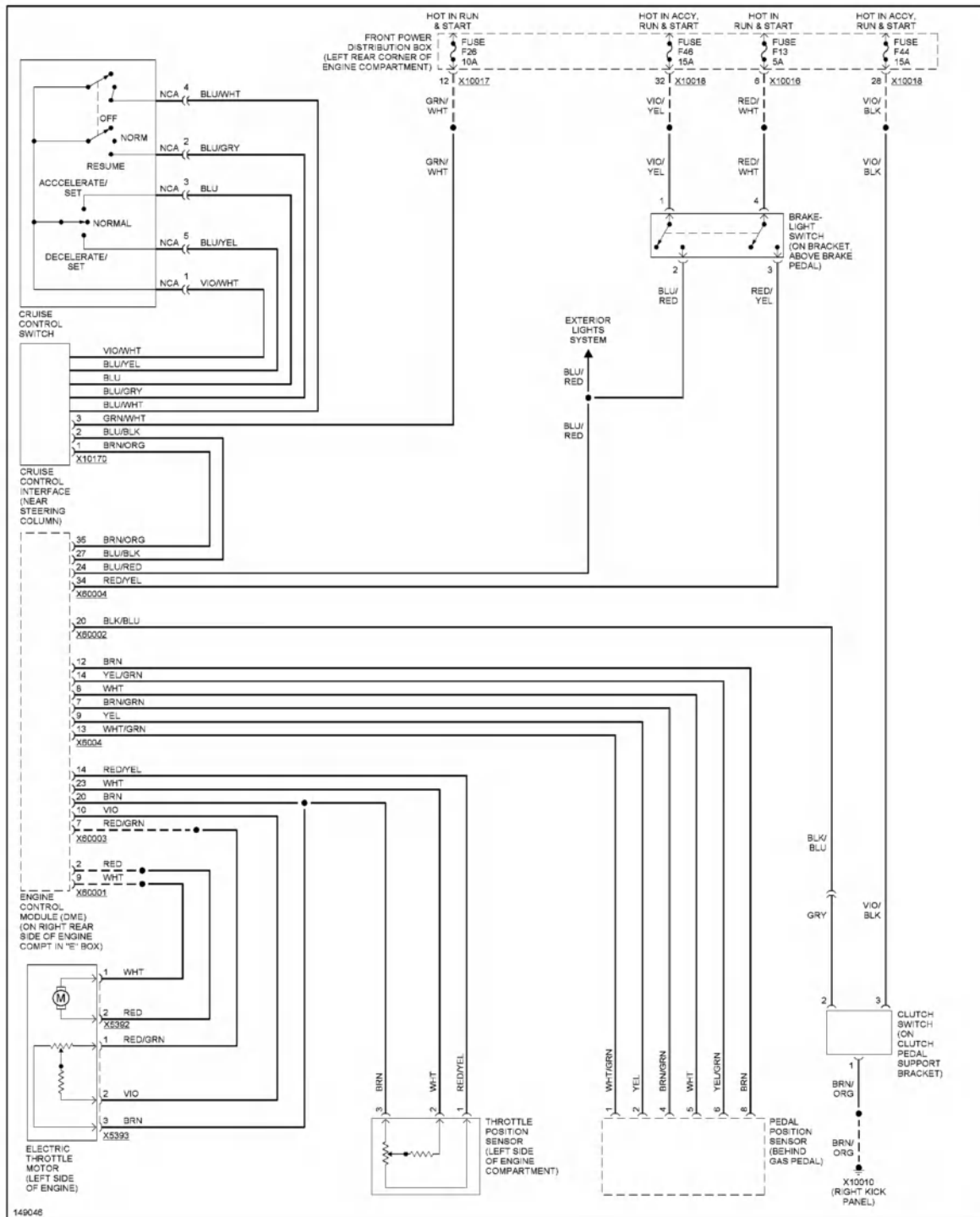
Fig. 14: Cruise Control Circuit, M-Versions
