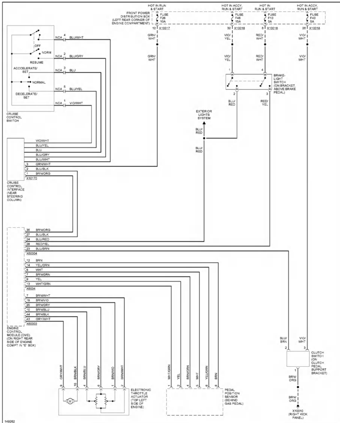
Fig. 15: Cruise Control Circuit, Z3 Versions
