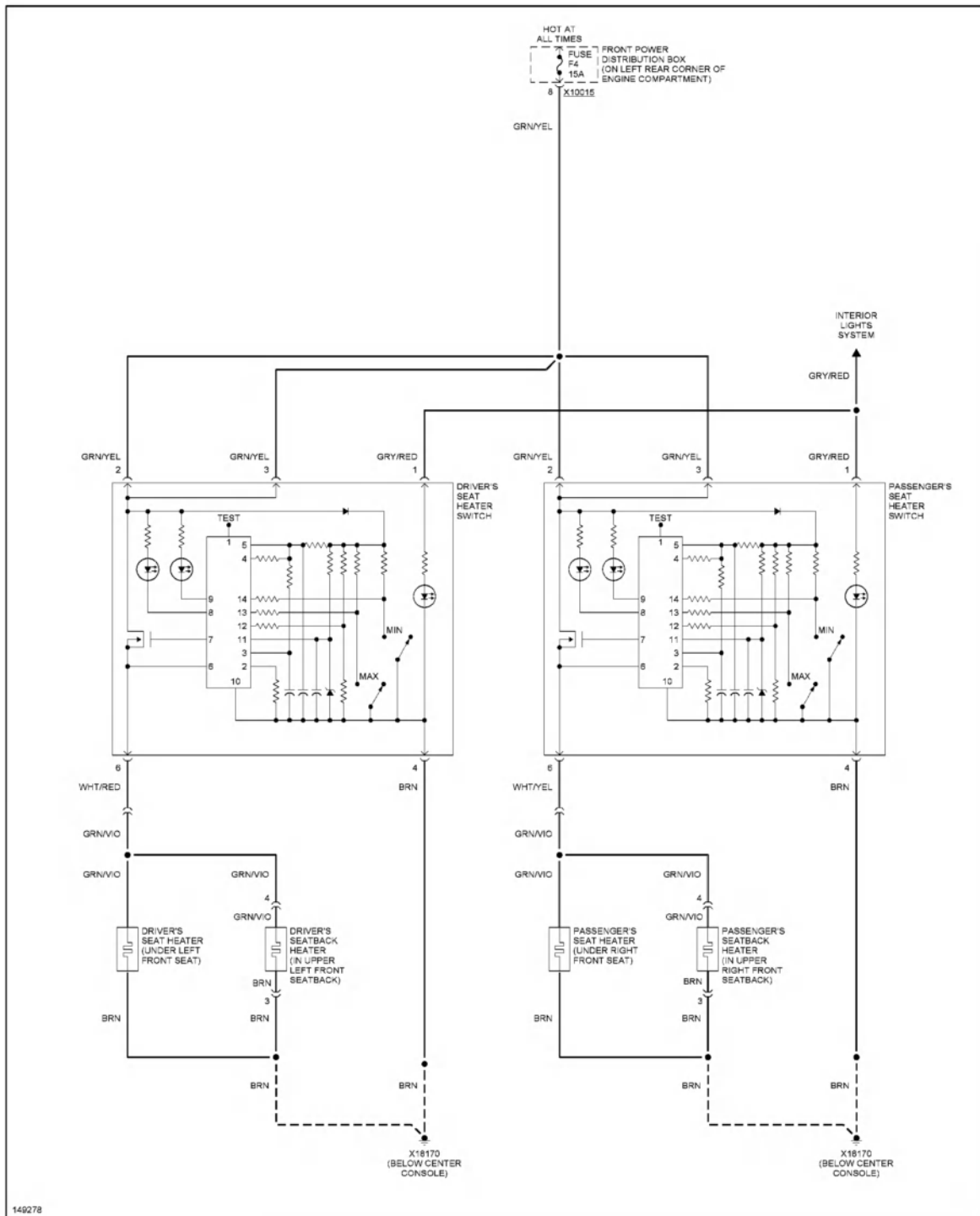
Fig. 56: Heated Seats Circuit
