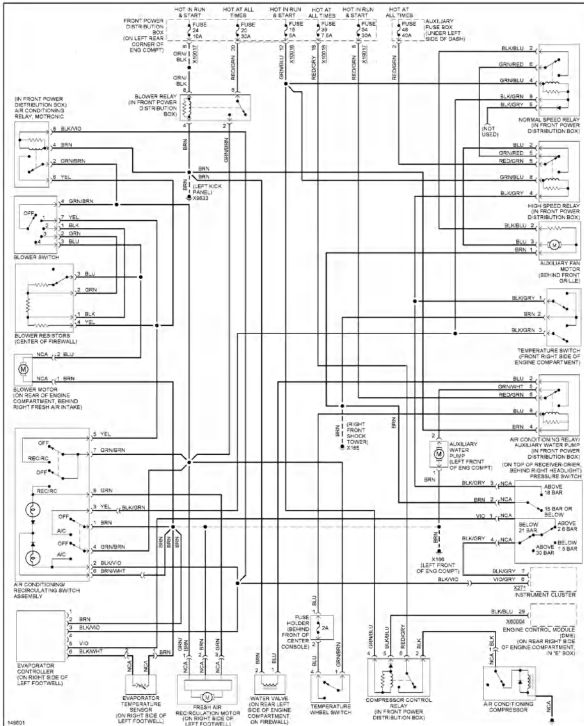
Fig. 1: Manual A/C Circuit, M-Versions
