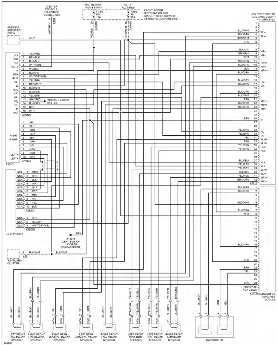
Fig. 63: Radio Circuit, Roadster W/ Harman Kardon
