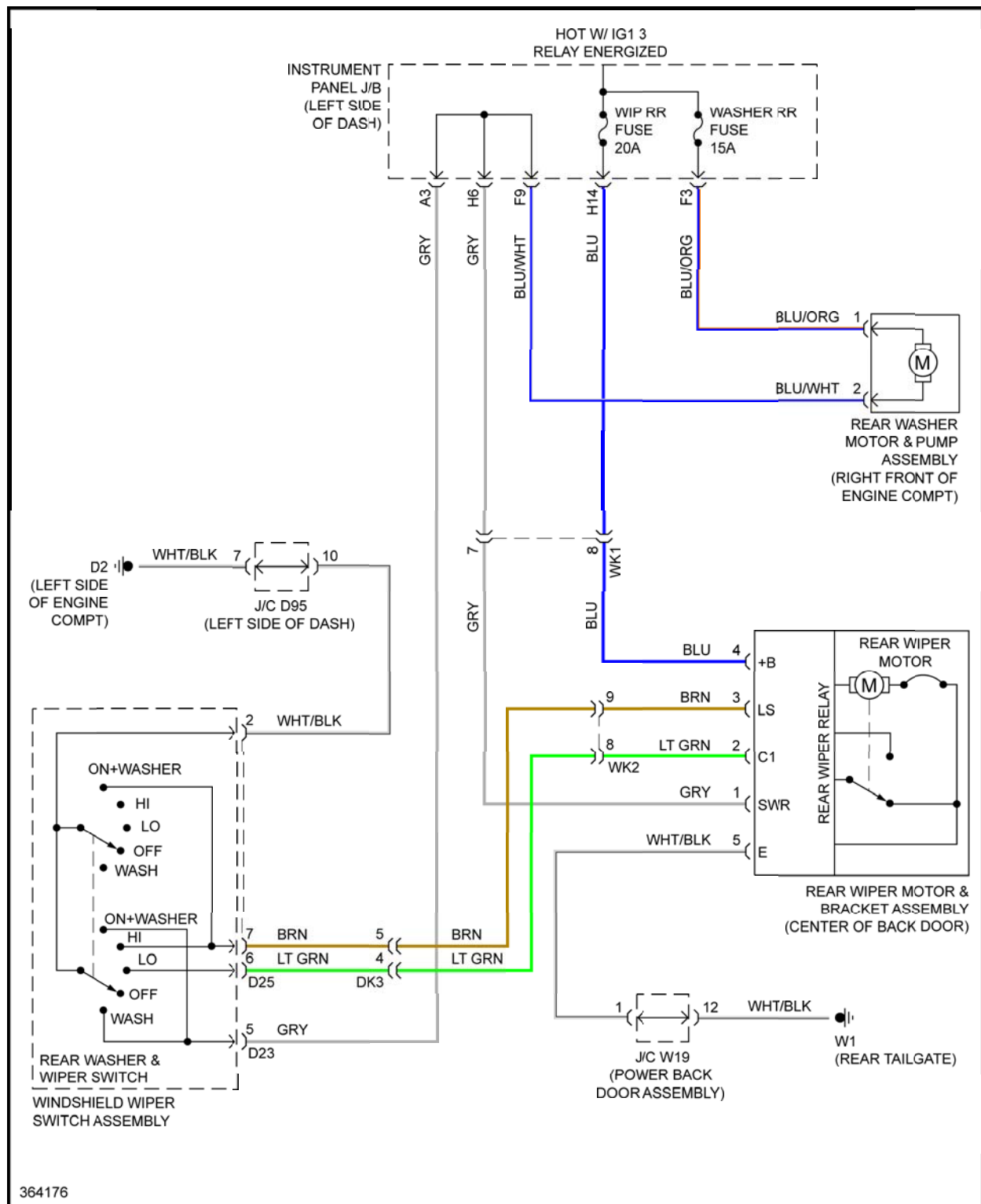
Fig. 128: Rear Wiper/Washer Circuit
