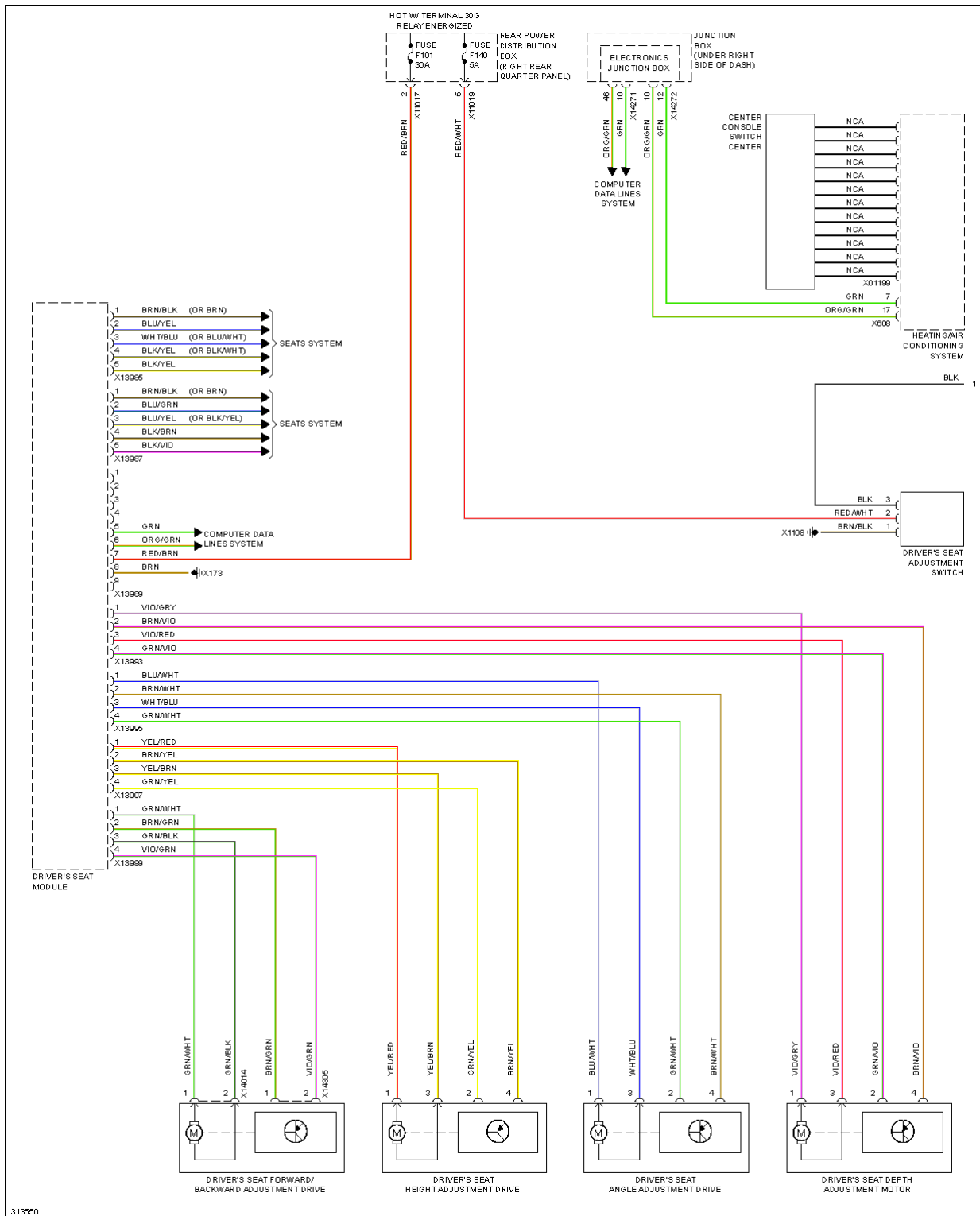
Fig. 59: Driver's Memory Seat Circuit, W/ Lumbar Support (1 of 2)
