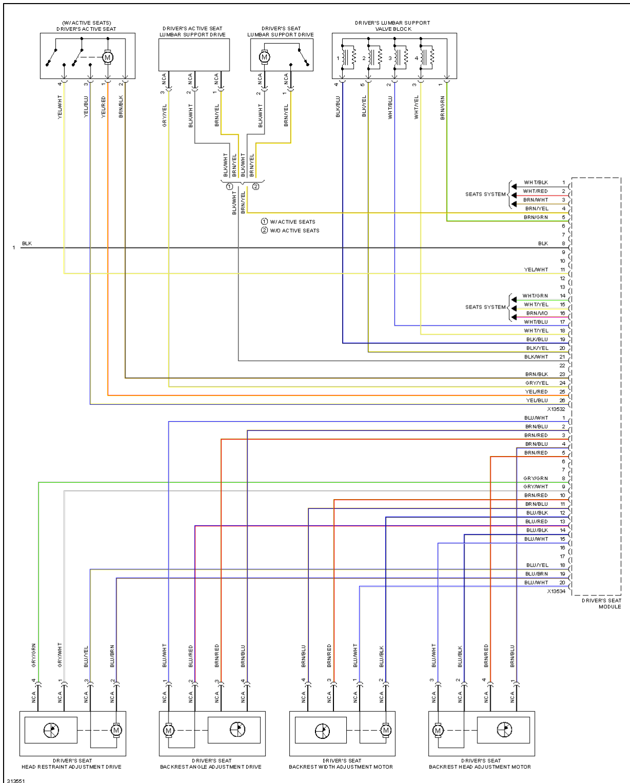
Fig. 60: Driver's Memory Seat Circuit, W/ Lumbar Support (2 of 2)
