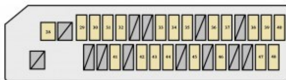
Scion tC mk1 – fuse box – instrument panel
