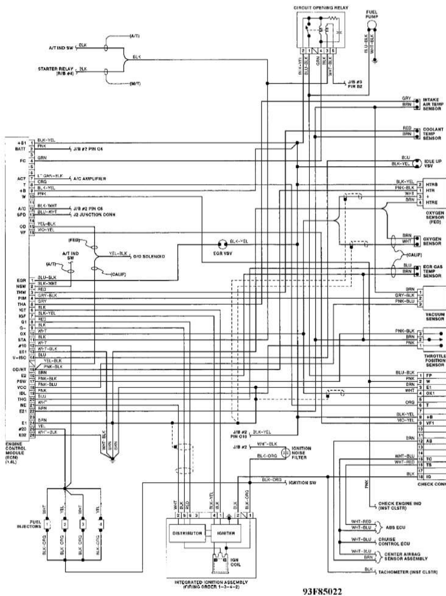
Fig. 1: Wiring Diagram (Celica 1.6L)
