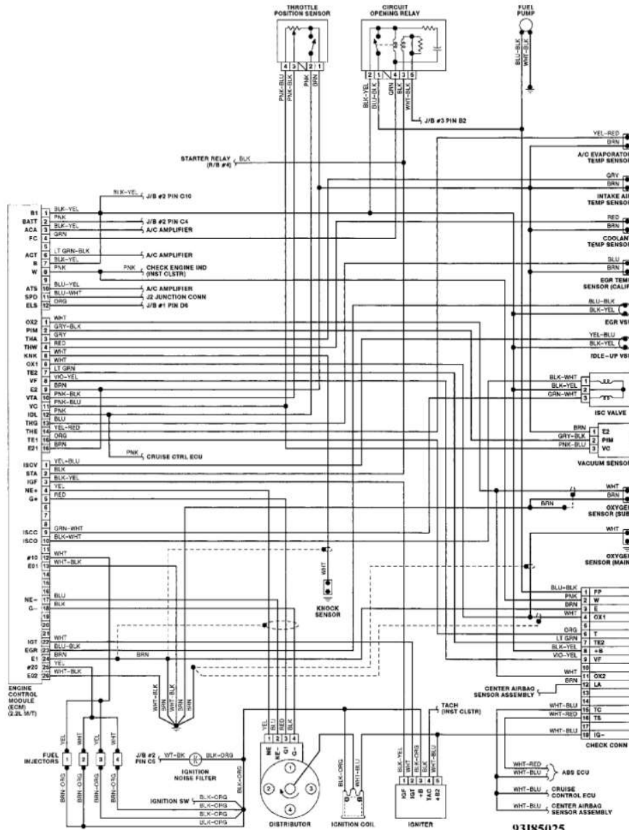
Fig. 4: Wiring Diagram (Celica 2.2L M/T)
