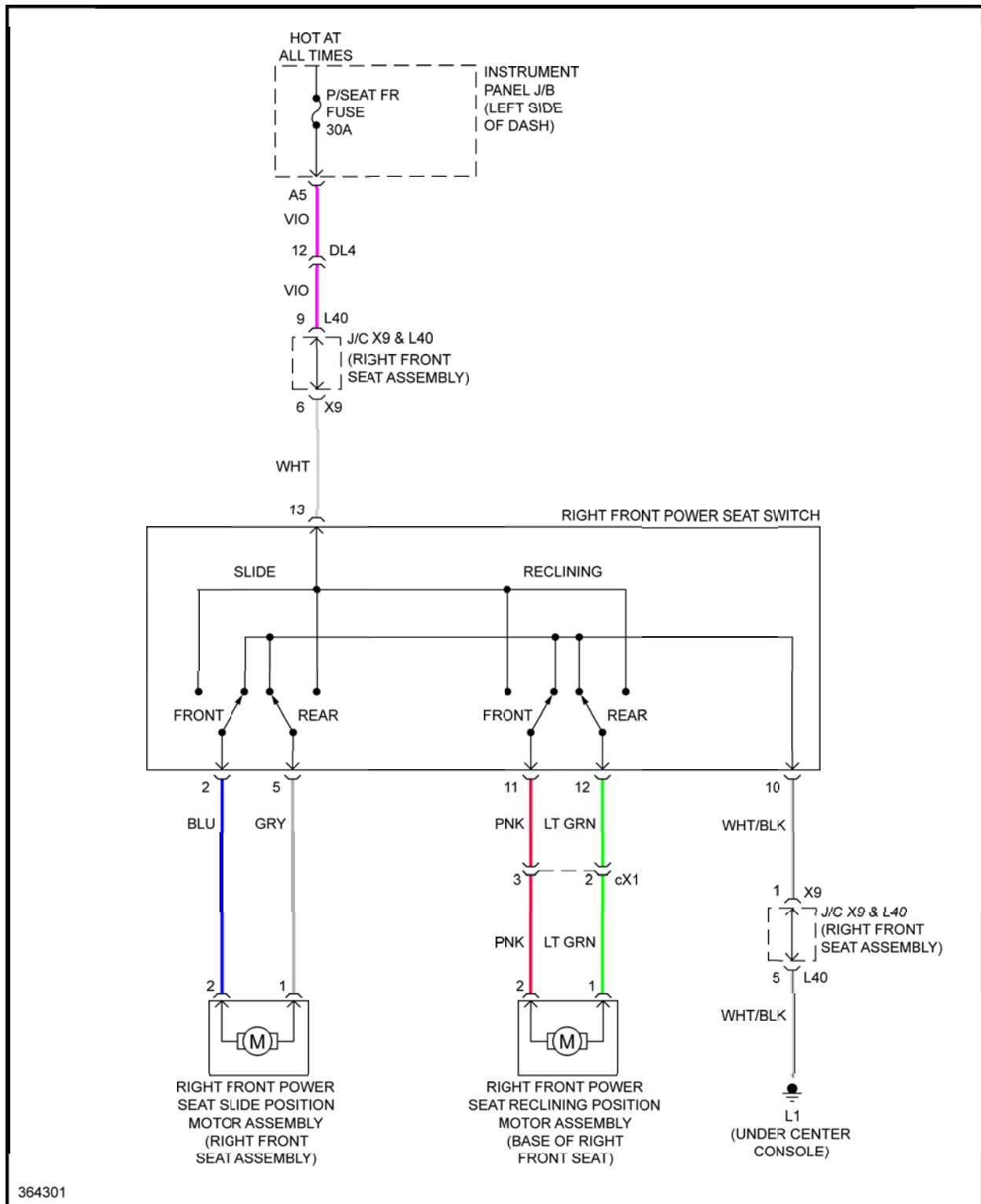
Fig. 86: Passenger Power Seat Circuit
