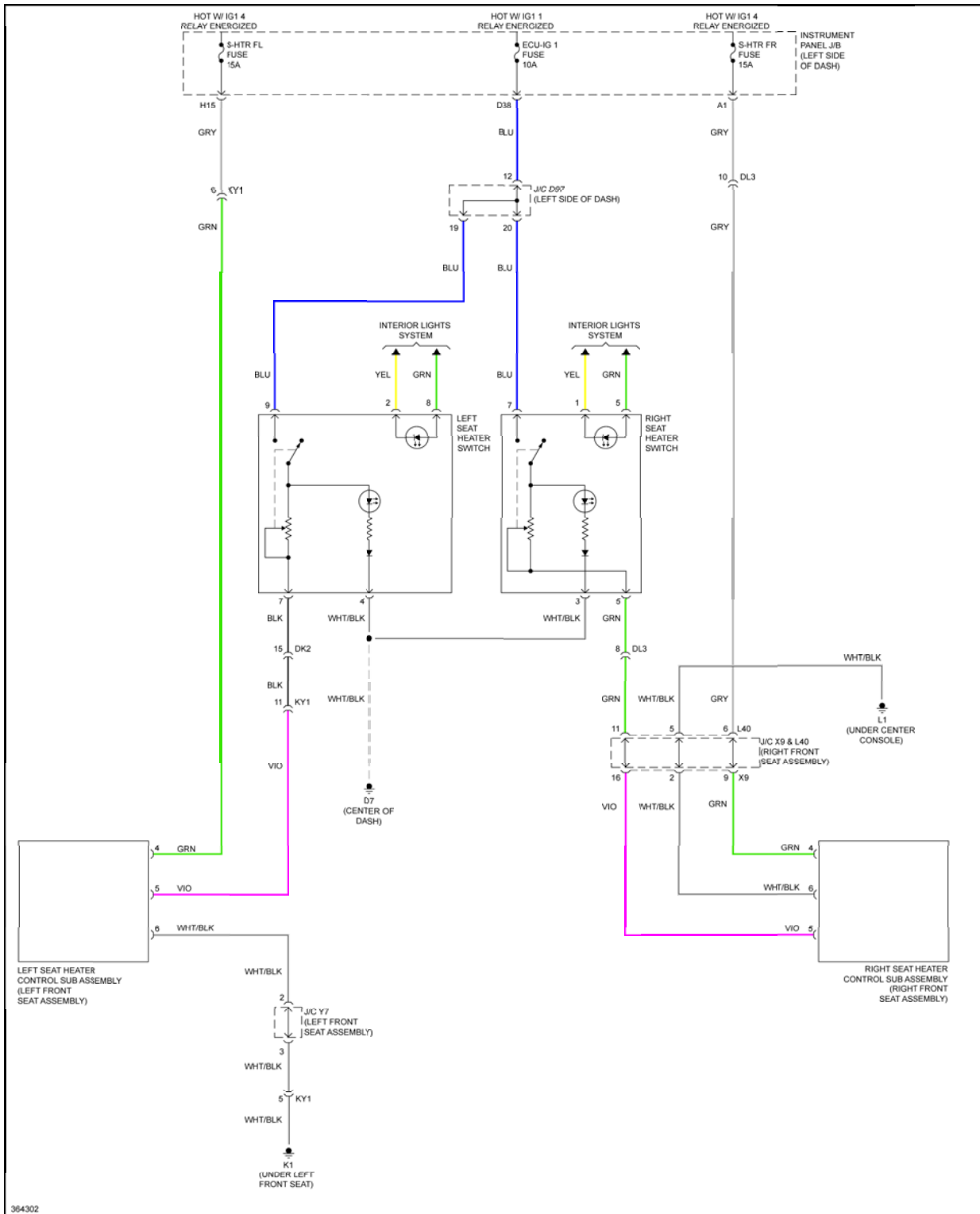
Fig. 85: Heated Seats Circuit
