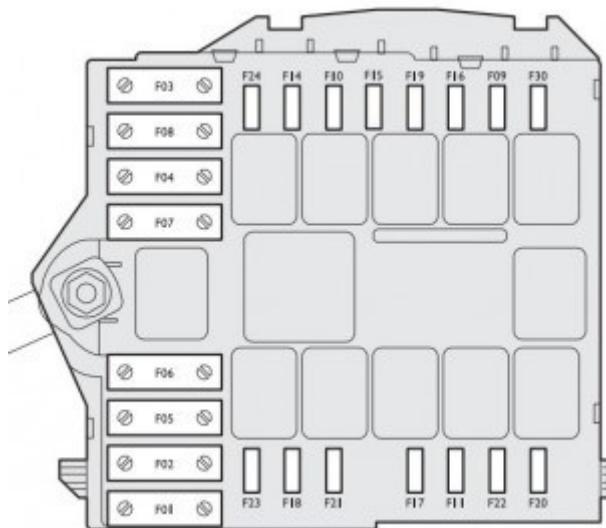
Fiat Stilo – fuse box – engine compartment (next to battery)
