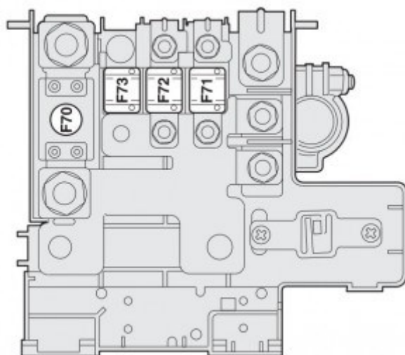
Fiat Stilo – fuse box – ob the battery positive pole
