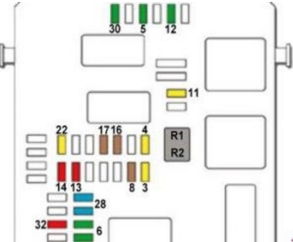
.Citroen C4 – fuse box diagram – instrument panel
