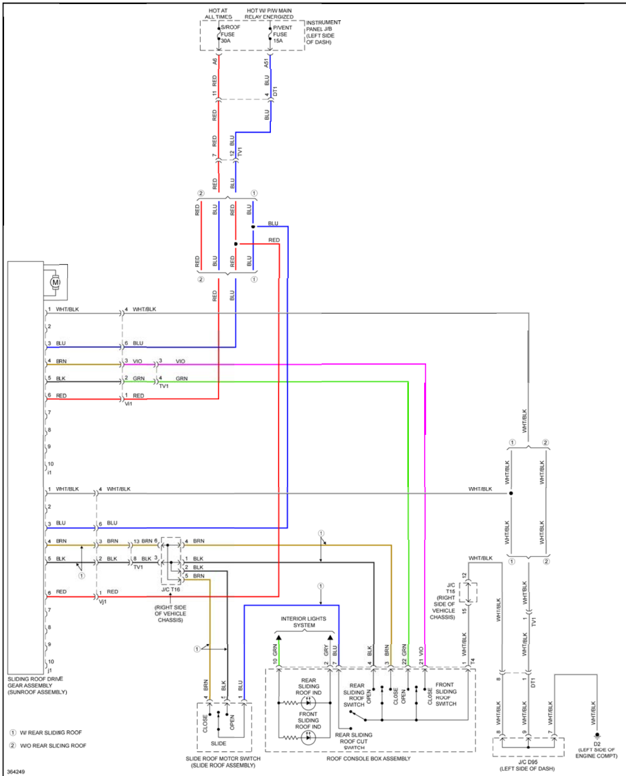
Fig. 89: Power Top/Sunroof Circuit
