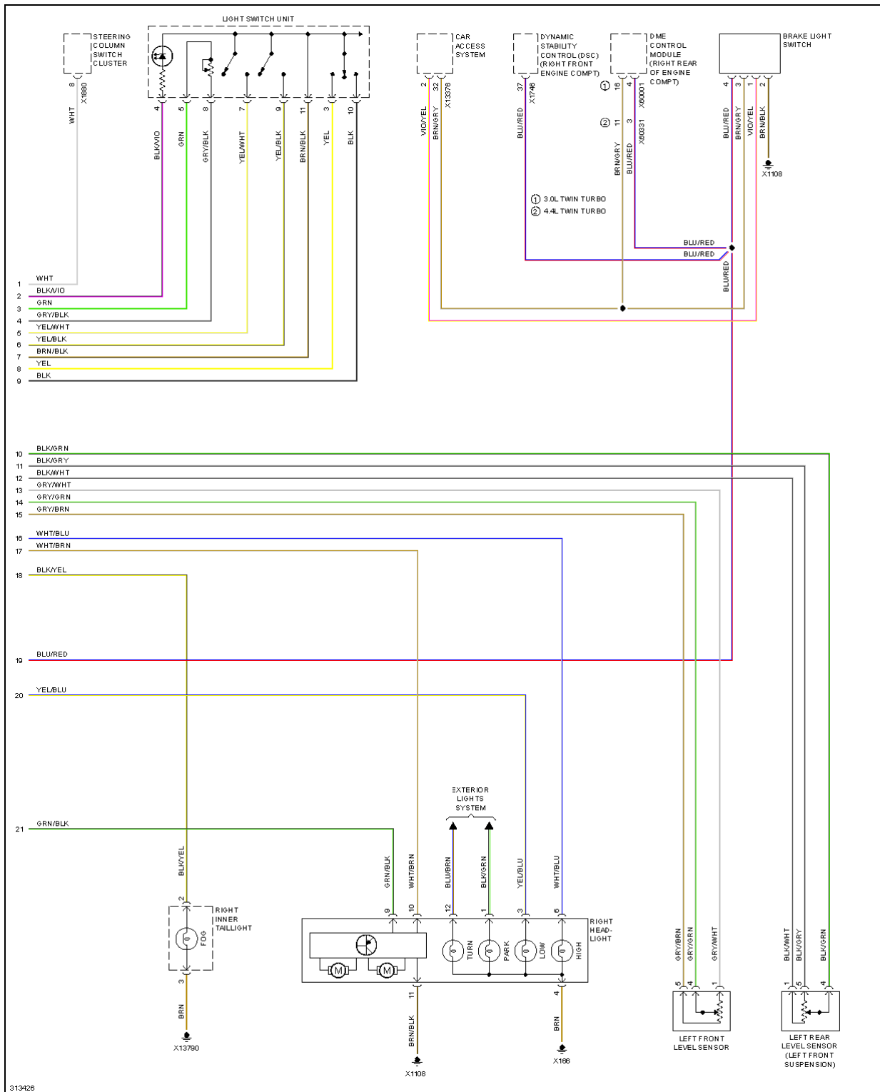
Fig. 51: Adaptive Front Lighting Circuit (2 of 2)
