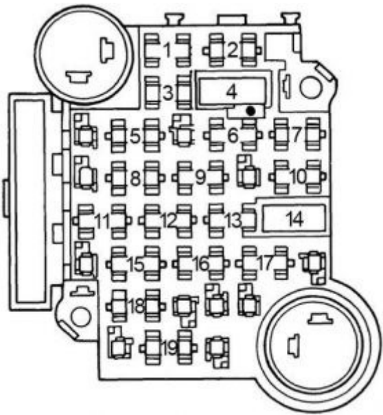
Buick Skylark – fuse box diagram
