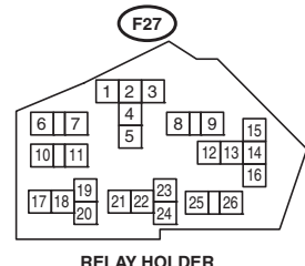
RELAY HOLDER
