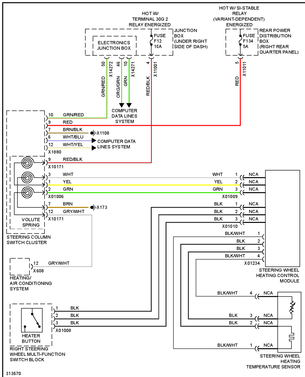
Fig. 93: Heated Steering Wheel Circuit
