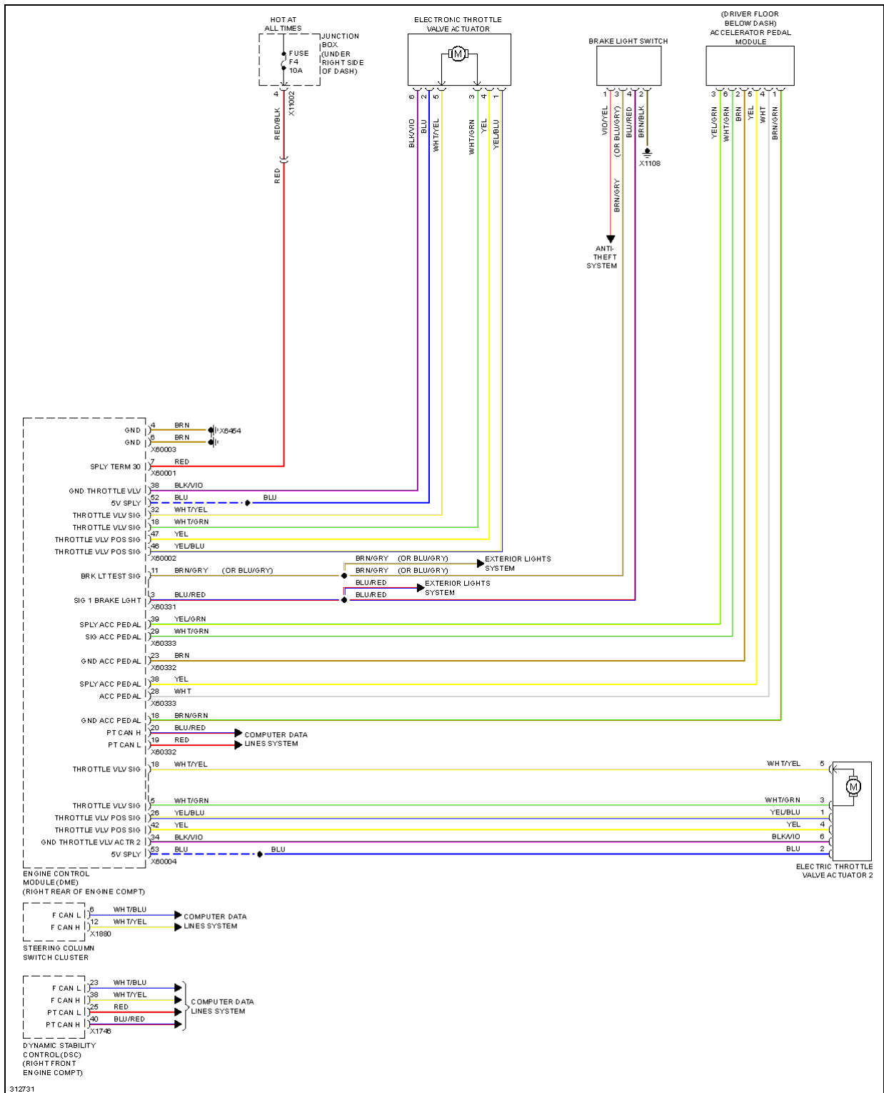
Fig. 23: 4.4L Twin Turbo, Cruise Control Circuit
