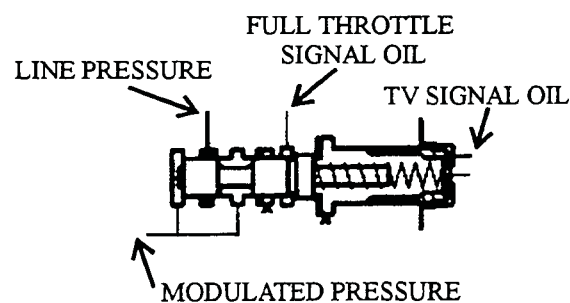
MODULATOR VALVE
