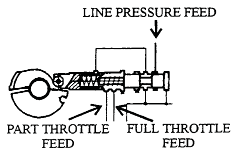
THROTTLE VALVE
