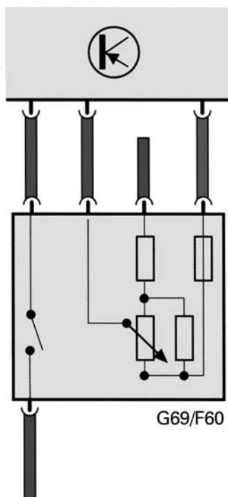
Electrical Circuit
