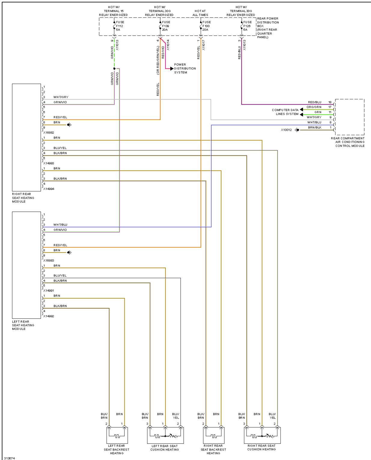
Fig. 97: Rear Heated Seats Circuit, W/ Rear A/C
