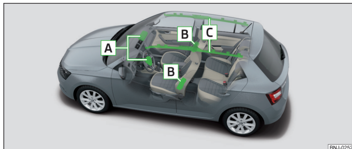
Fig. 19 Airbag installation points
