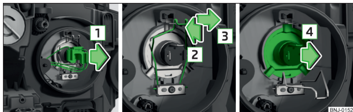
Fig. 299 Removing bulbs for low and main beam
