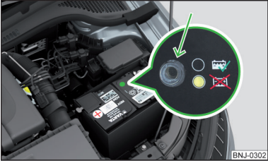
Fig. 263 Vehicle battery: Electrolyte level indicator
