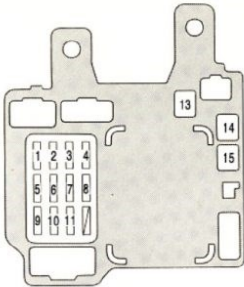
Lexus ES300 – fuse box – instrument panel
