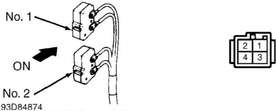
Fig. 2: Limit Switch Terminal ID Courtesy of Toyota Motor Sales, U.S.A., Inc.
