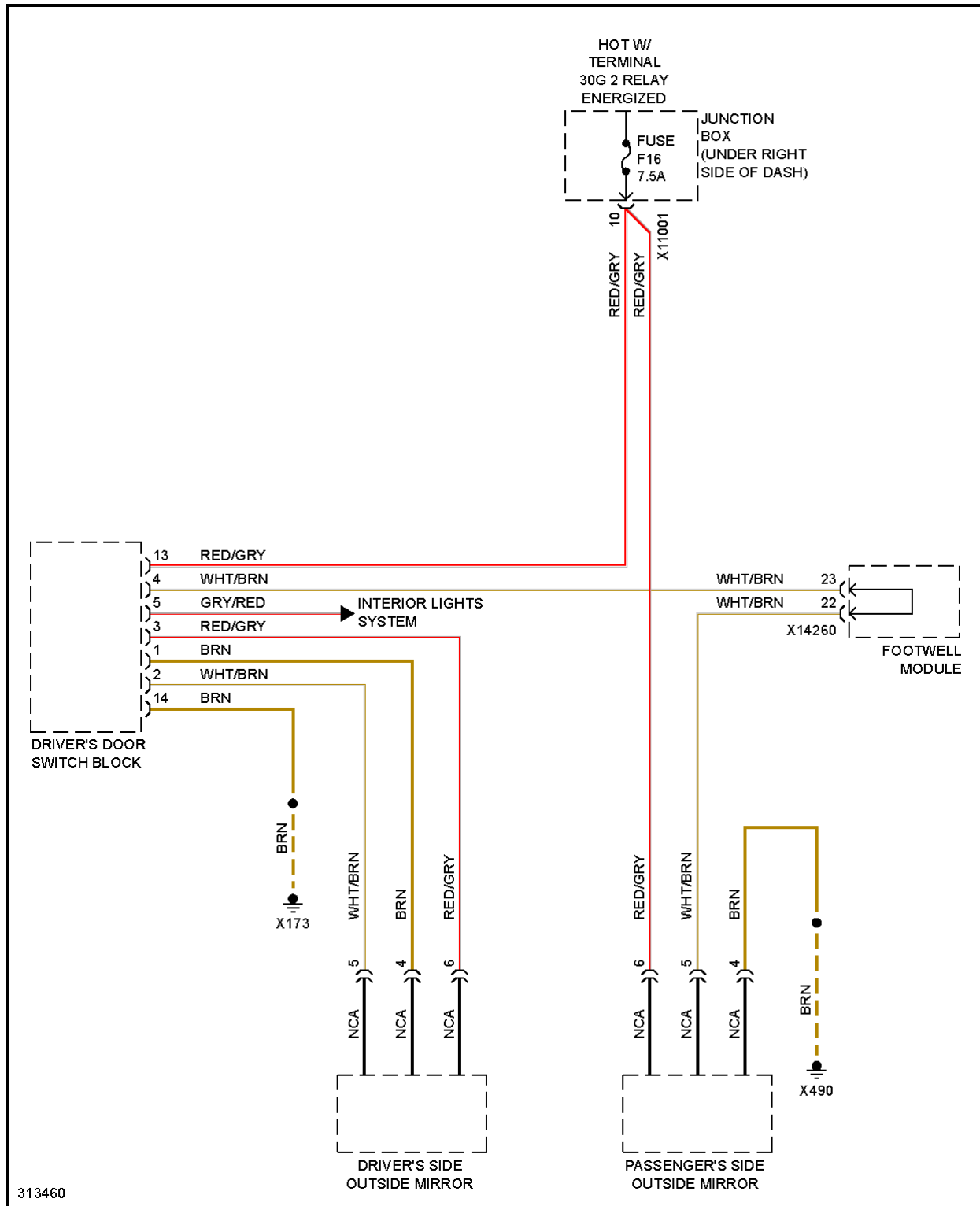
Fig. 24: Heated Mirrors Circuit, W/ LIN bus Function
