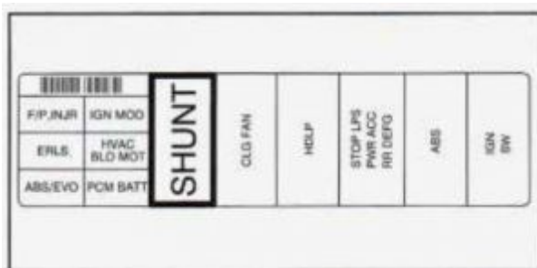
Buick Skylark – fuse box – engine compartment
