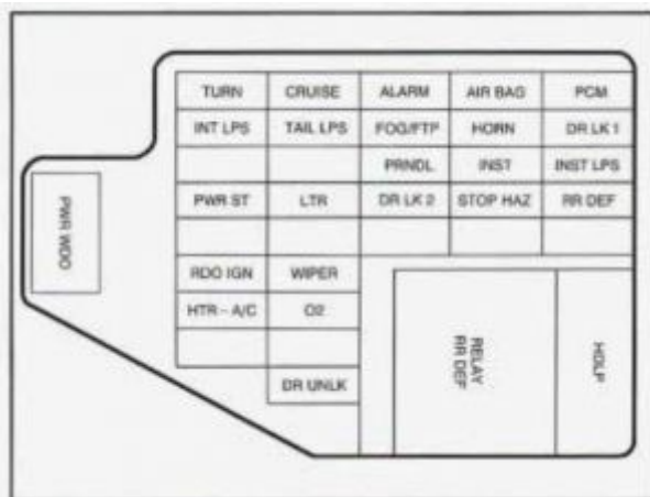
Buick Skylark – fuse box – instrument panel
