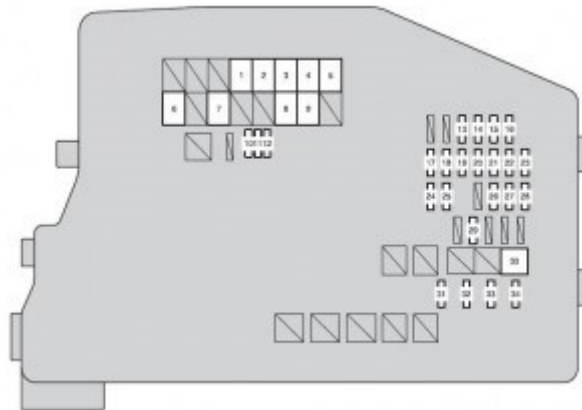
Scion tC mk2 – fuse box – engine compartment
