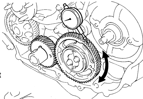
Oil Pump x Crankshaft
