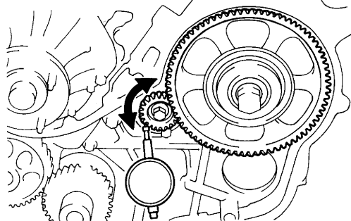
Balanceshaft No.2 x Injection Pump
