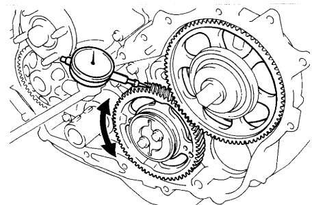
Injection Pump x Idler
