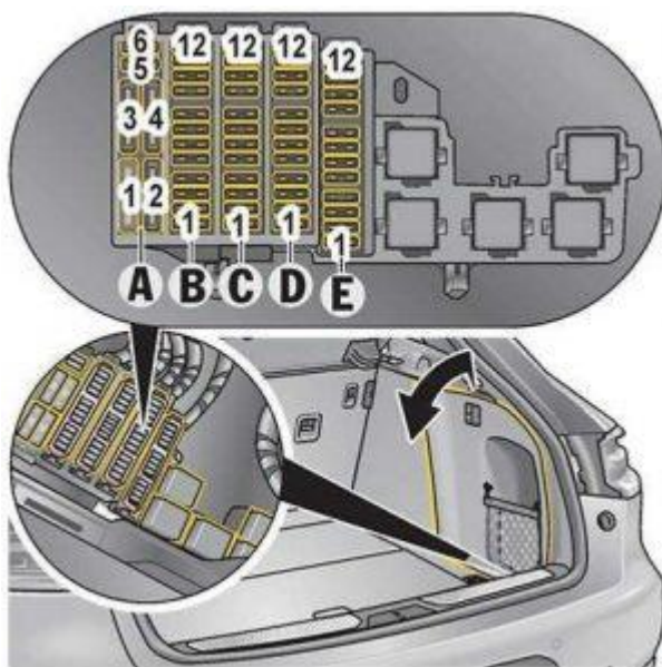
Porsche Macan – fuse box diagram –
