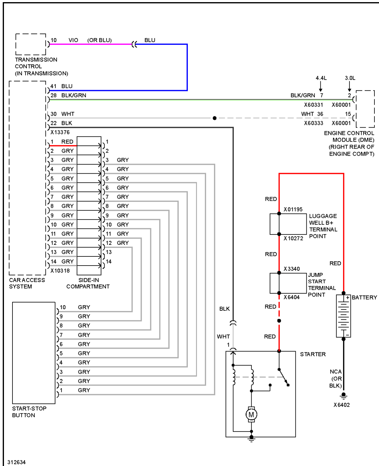
Fig. 119: Starting Circuit
