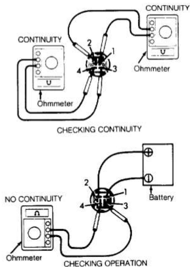
93E84024 Fig. 2: Testing Cooling Fan Relay No. 1 & Engine Compartment Cooling Fan Relay Courtesy of Toyota Motor Sales, U.S.A., Inc.
