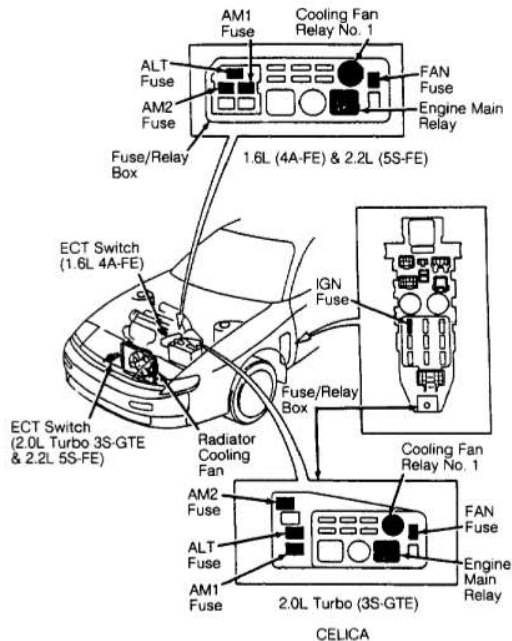
93D84015 Fig. 1: Identifying Radiator Cooling Fan & Components Courtesy of Toyota Motor Sales, U.S.A., Inc.
