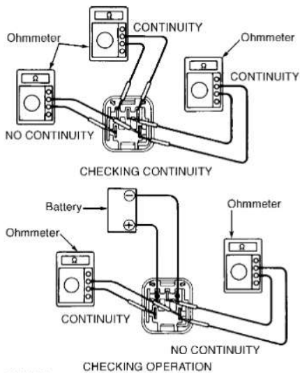
Fig. 3: Testing Engine Main Relay Courtesy of Toyota Motor Sales, U.S.A., Inc.
