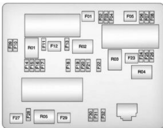
Buick Verano – fuse box – rear compartment
