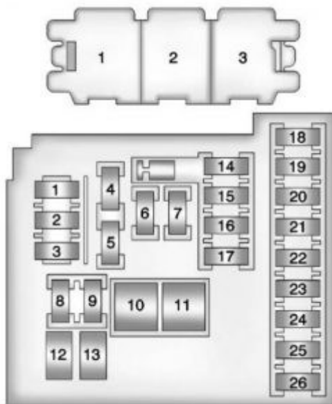
Buick Verano – fuse box – instrument panel
