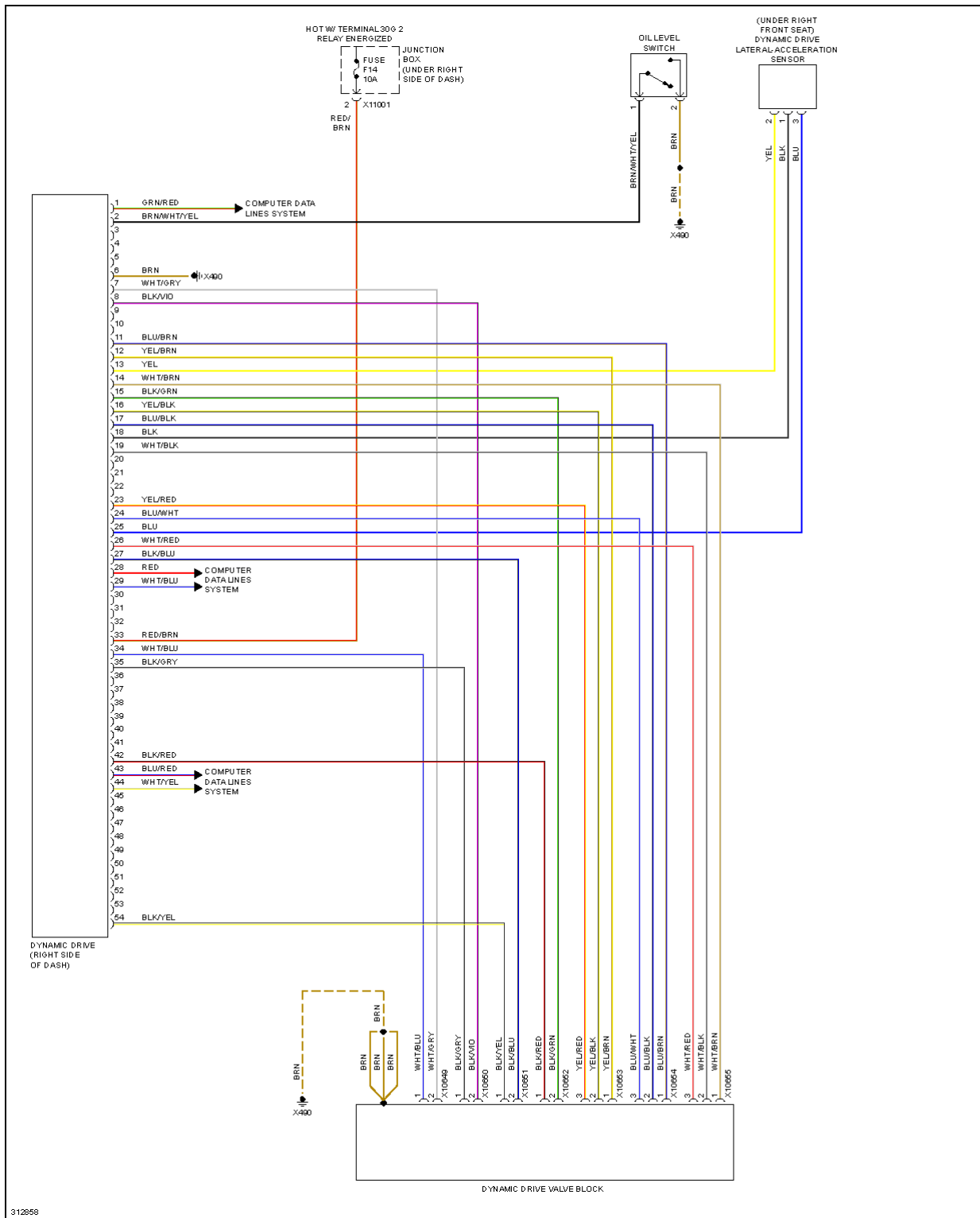
Fig. 30: Dynamic Drive Suspension Circuit
