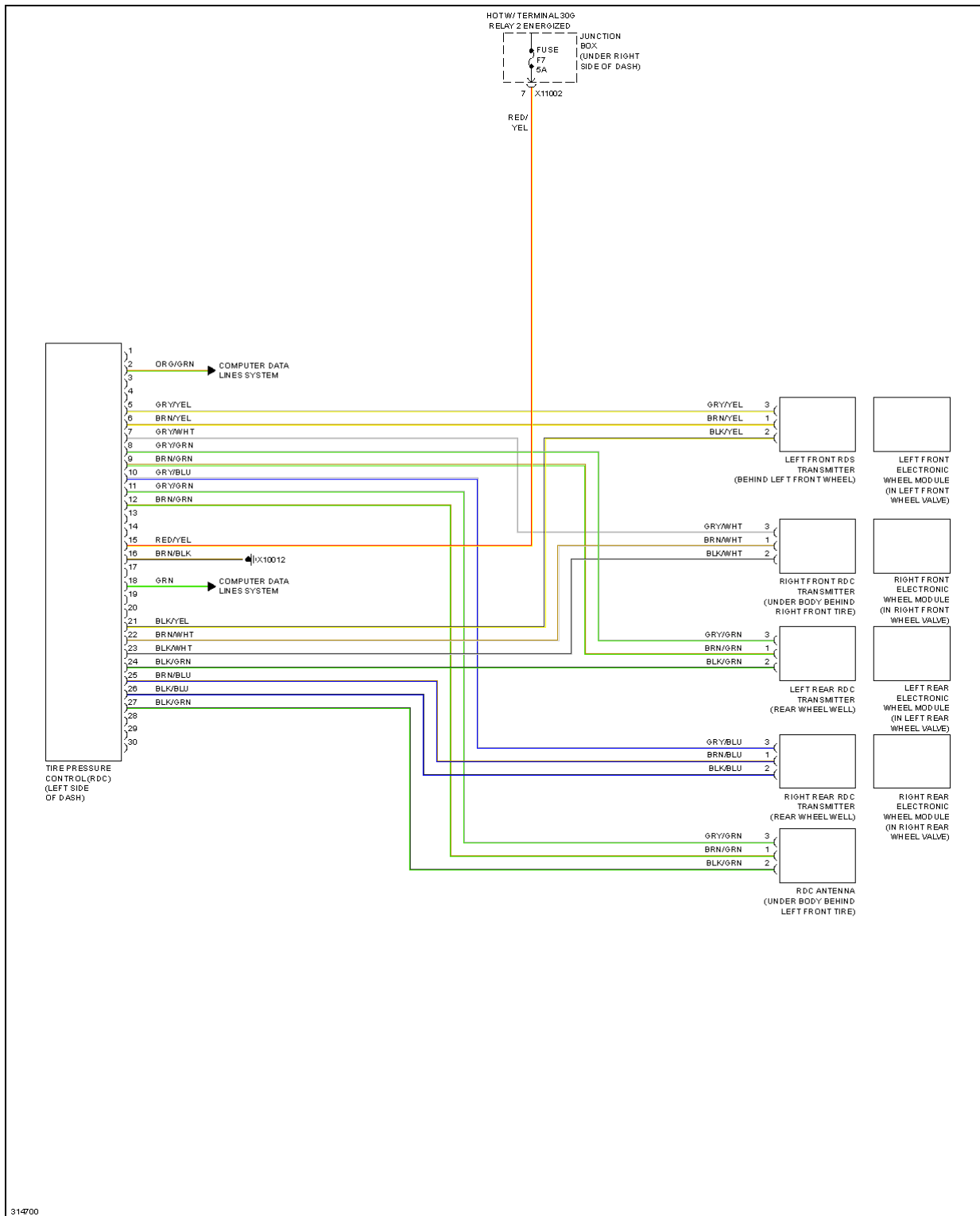
Fig. 128: Warning Systems Circuit
